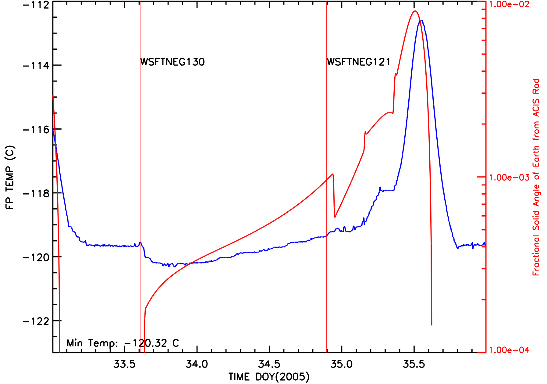
ACIS Focal Plane Temperature vs Time [02/02-05/06]
