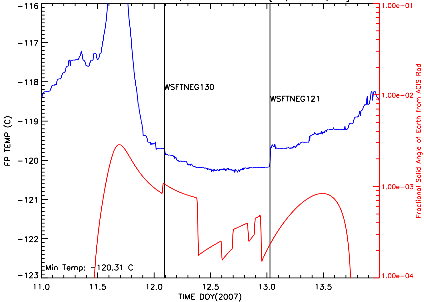
ACIS Focal Plane Temperature vs Time [01/11-14/07]
