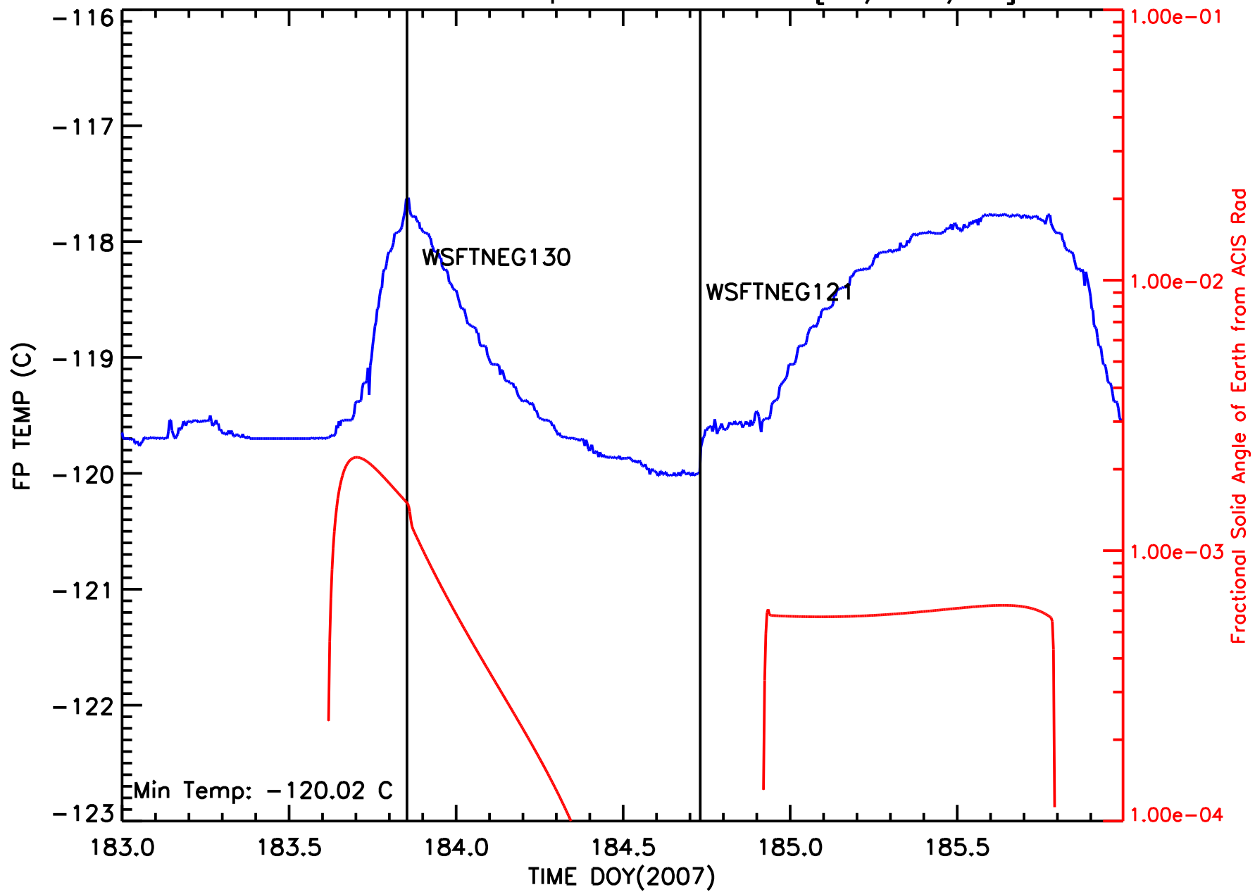
ACIS Focal Plane Temperature vs Time [07/2-5/07]
