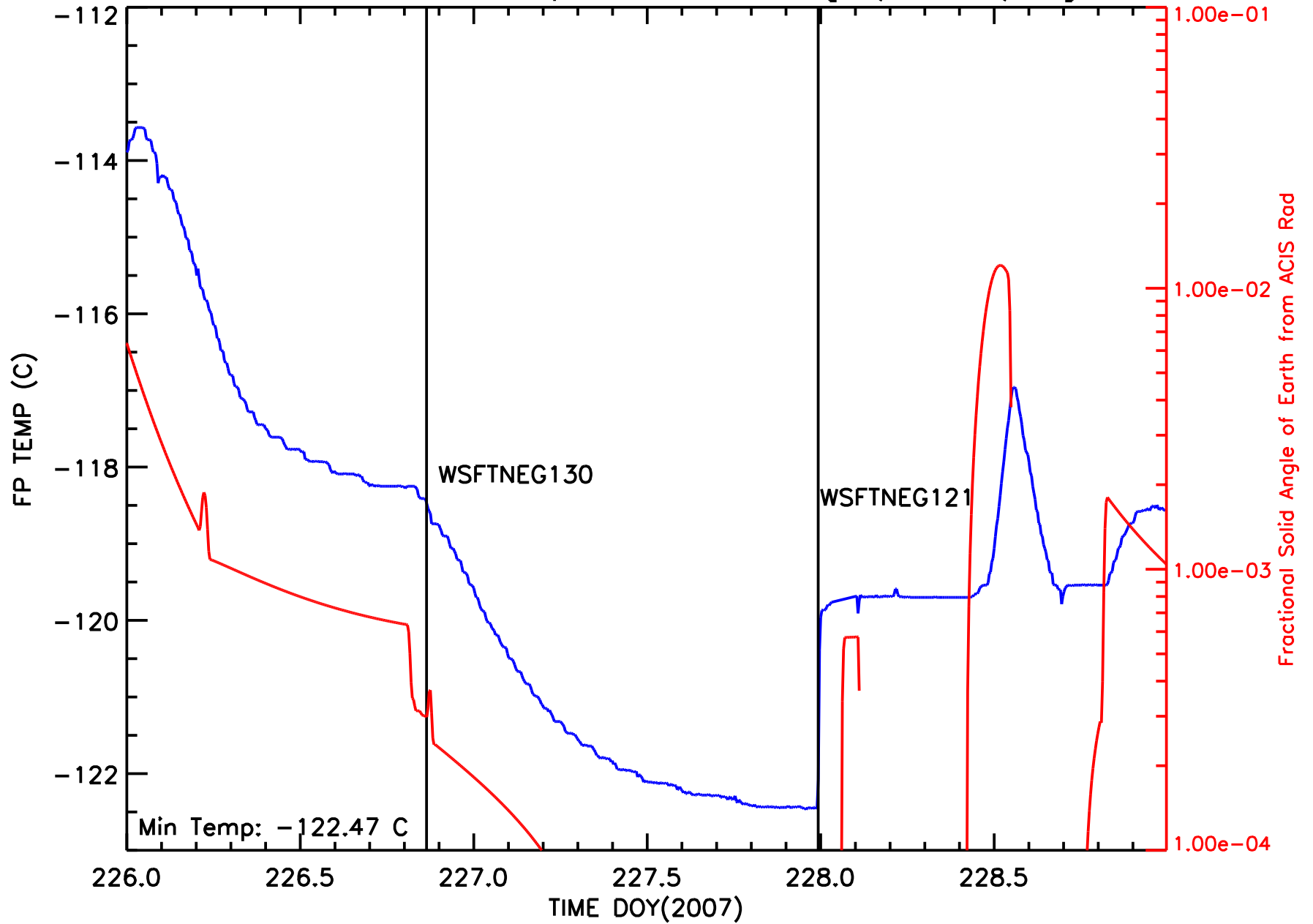
ACIS Focal Plane Temperature vs Time [08/14-17/07]
