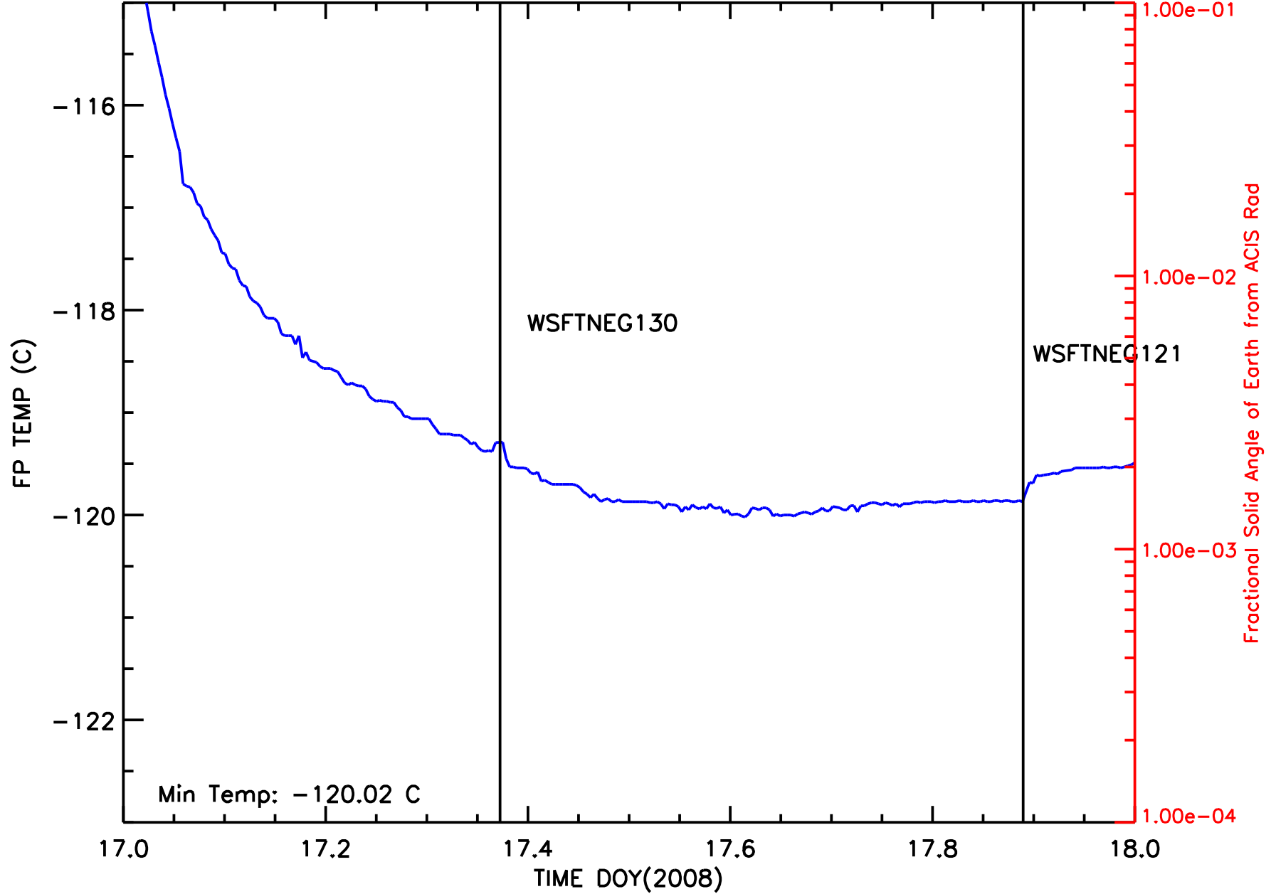
ACIS Focal Plane Temperature vs Time [01/17-18/08]
