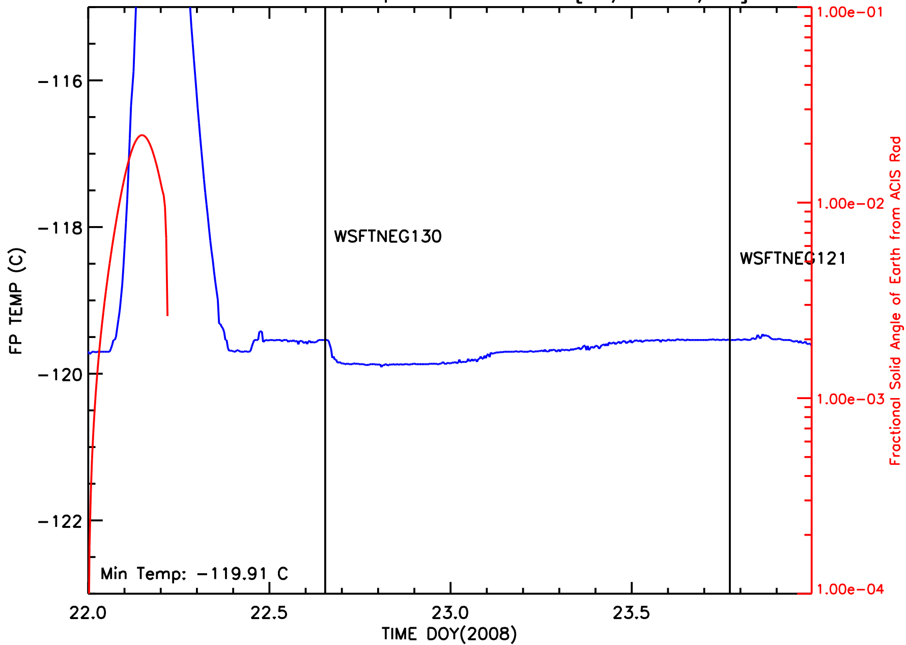
ACIS Focal Plane Temperature vs Time [01/22-24/08]
