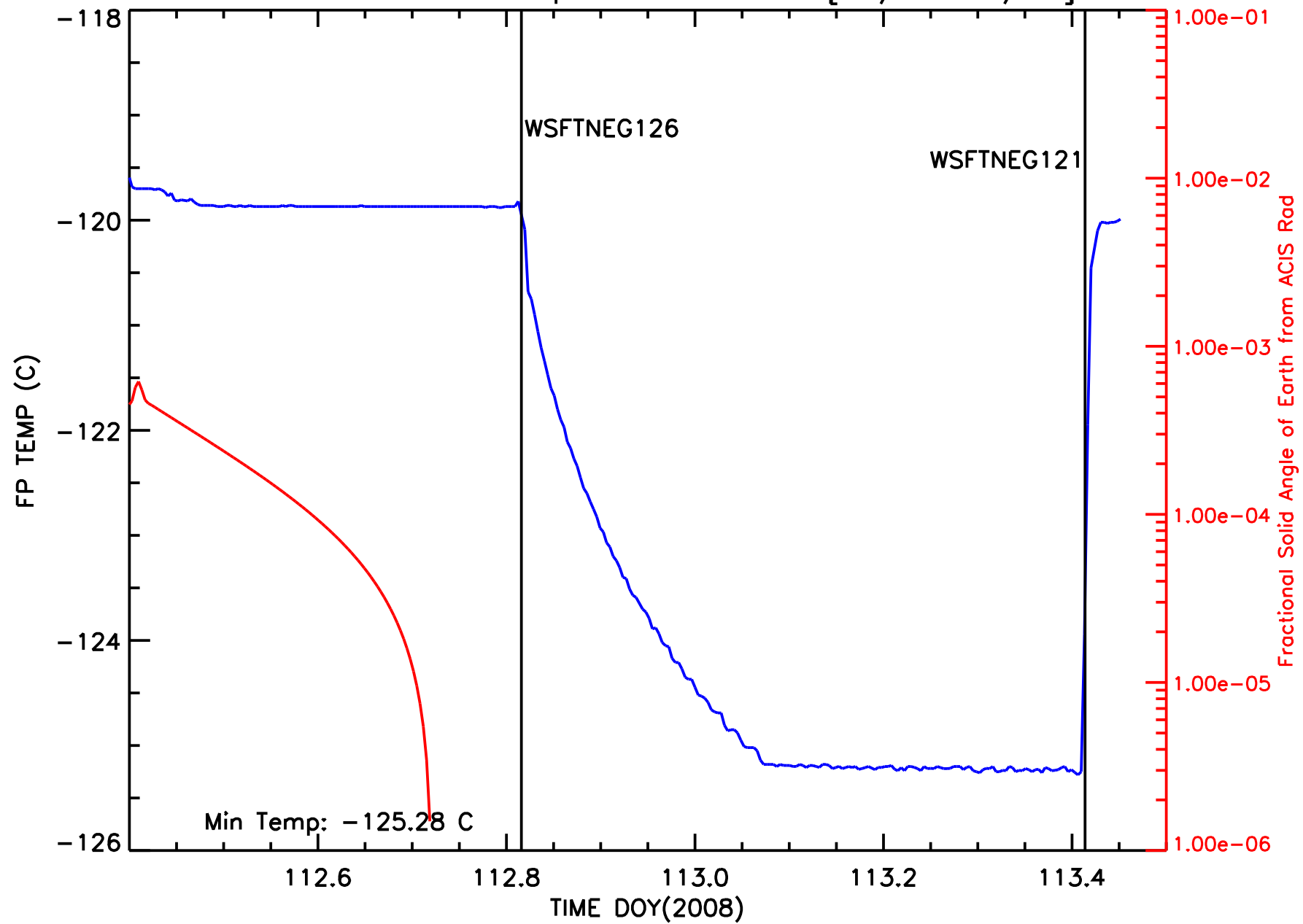
ACIS Focal Plane Temperature vs Time [04/21-23/08]
