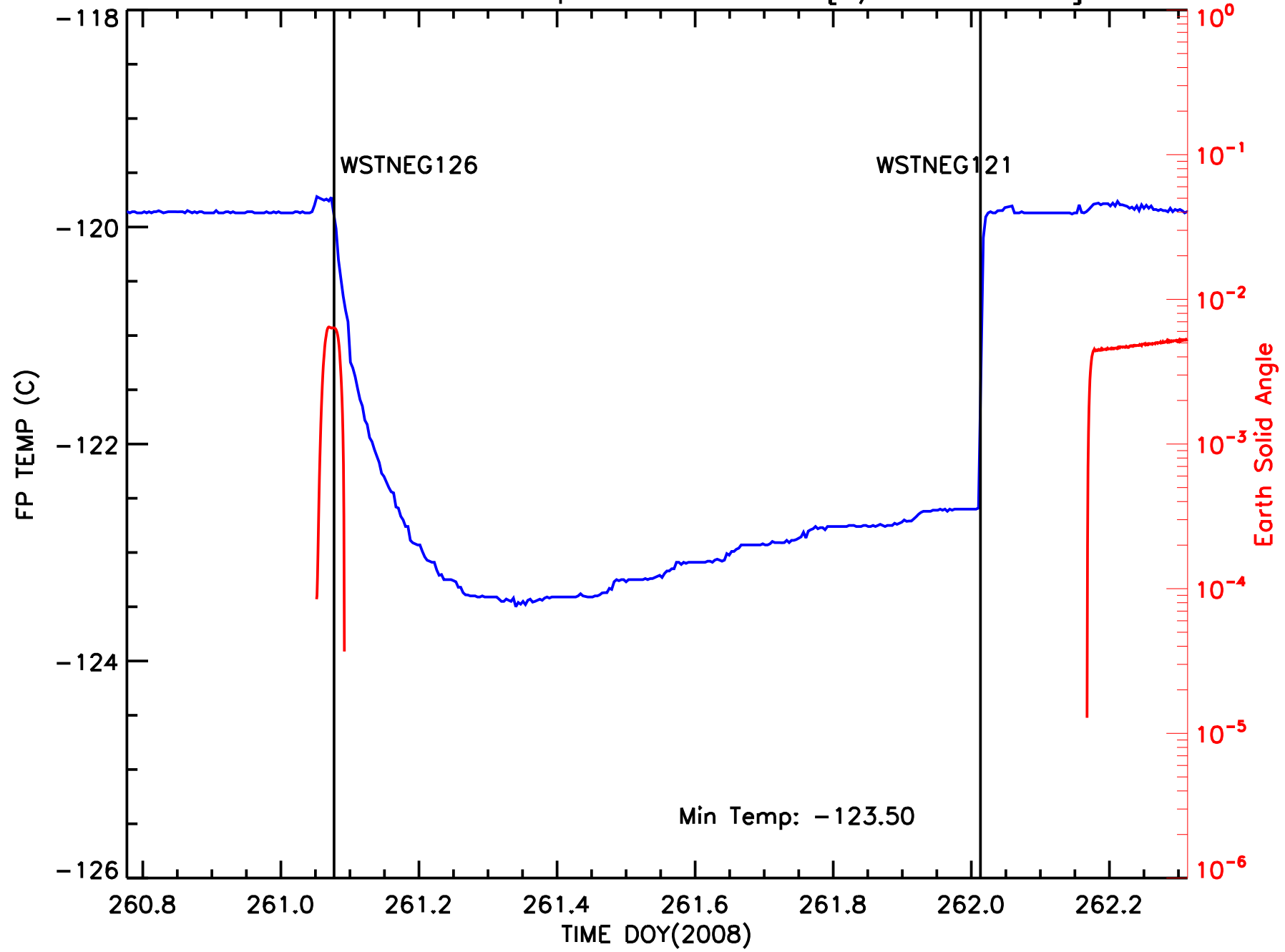
ACIS Focal Plane Temperature vs Time [9/18-19 2008]
