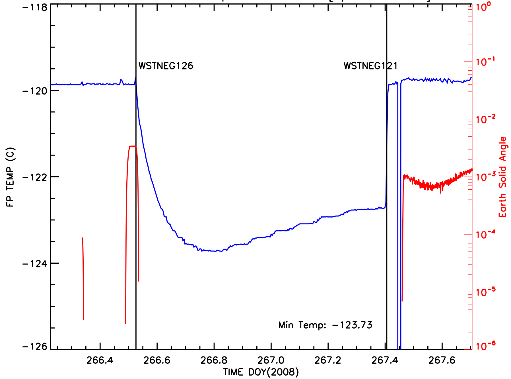
ACIS Focal Plane Temperature vs Time [9/23-24 2008]
