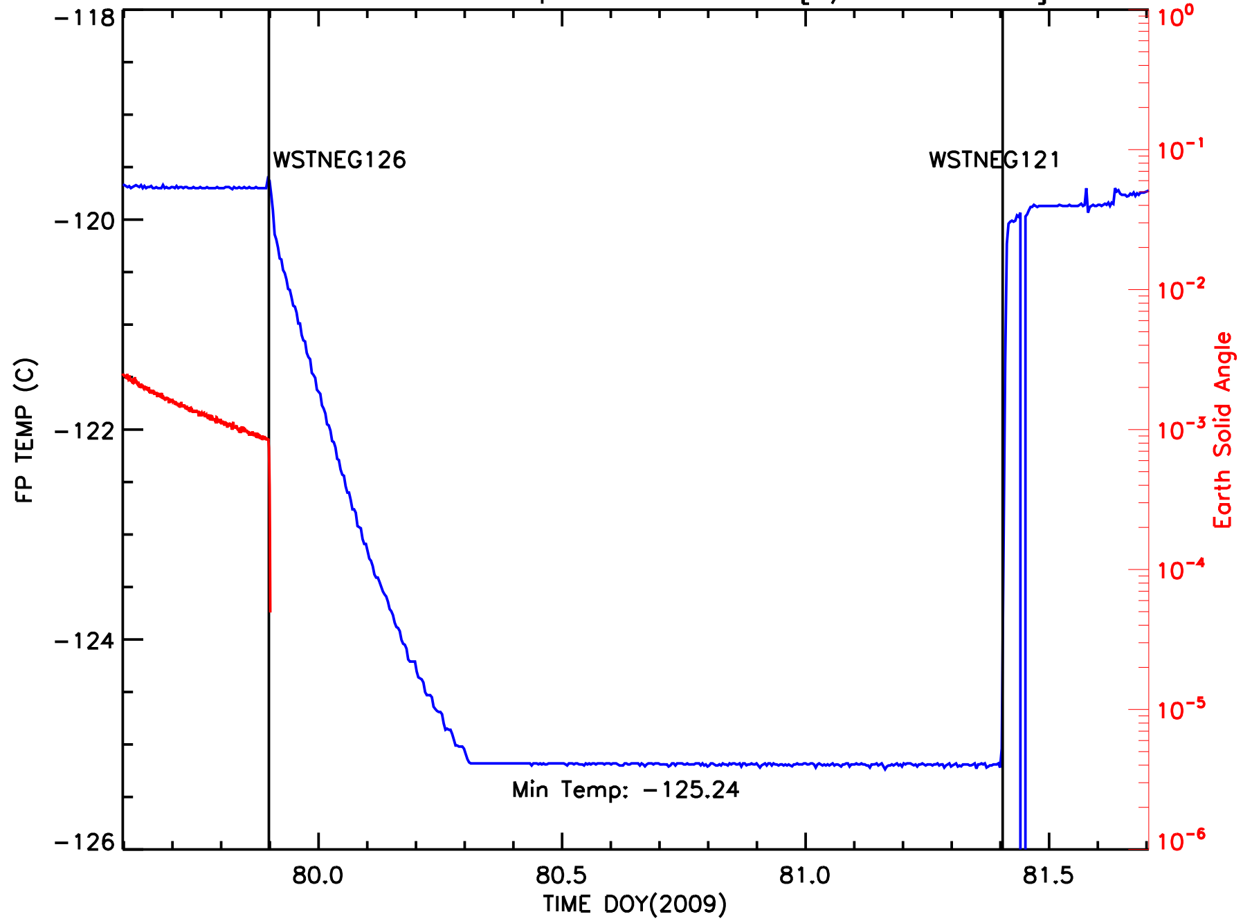
ACIS Focal Plane Temperature vs Time [3/20-22 2009]
