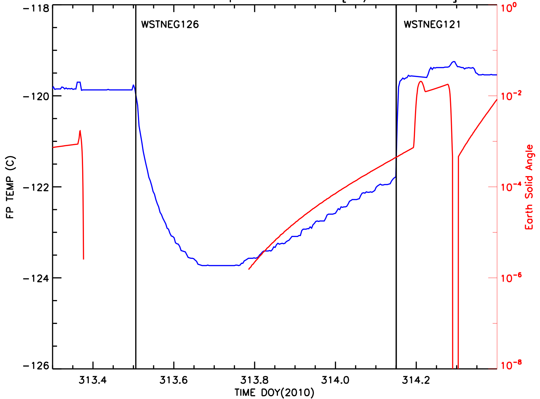
ACIS Focal Plane Temperature vs Time [11/09-10 2010]
