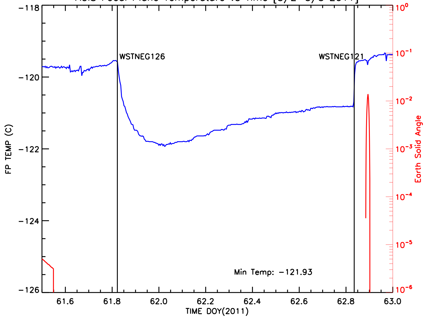
ACIS Focal Plane Temperature vs Time [3/2-3/3 2011]
