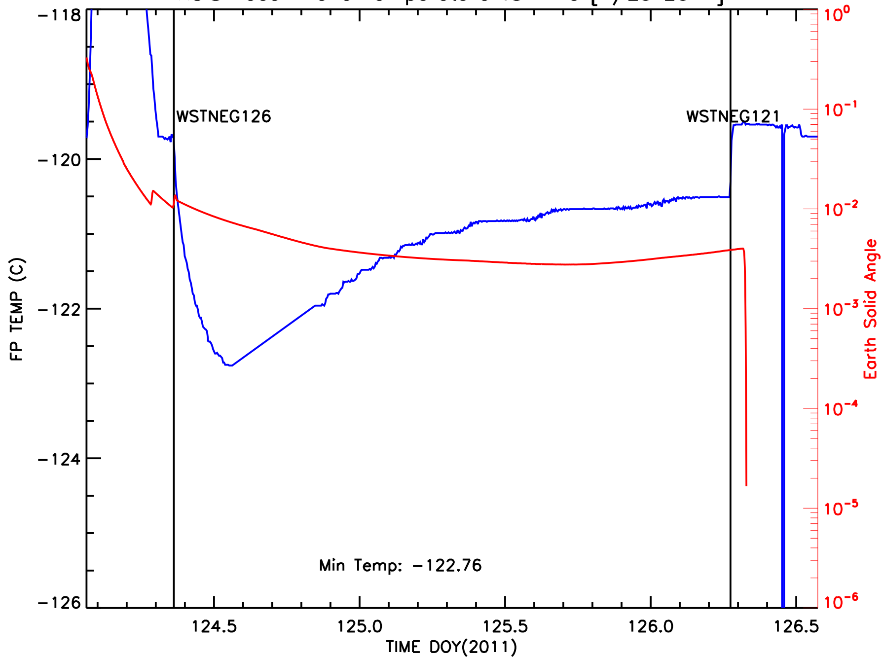
ACIS Focal Plane Temperature vs Time [4/29 2011]
