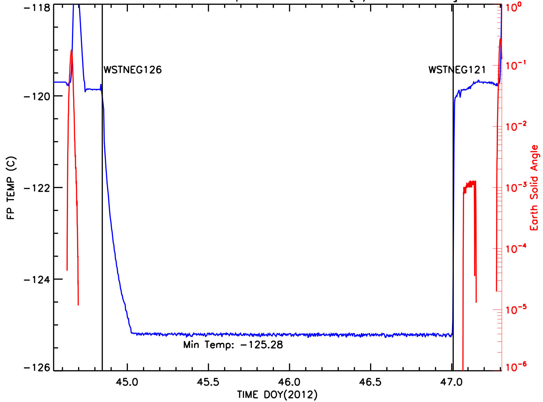
ACIS Focal Plane Temperature vs Time [2/13-16 2012]
