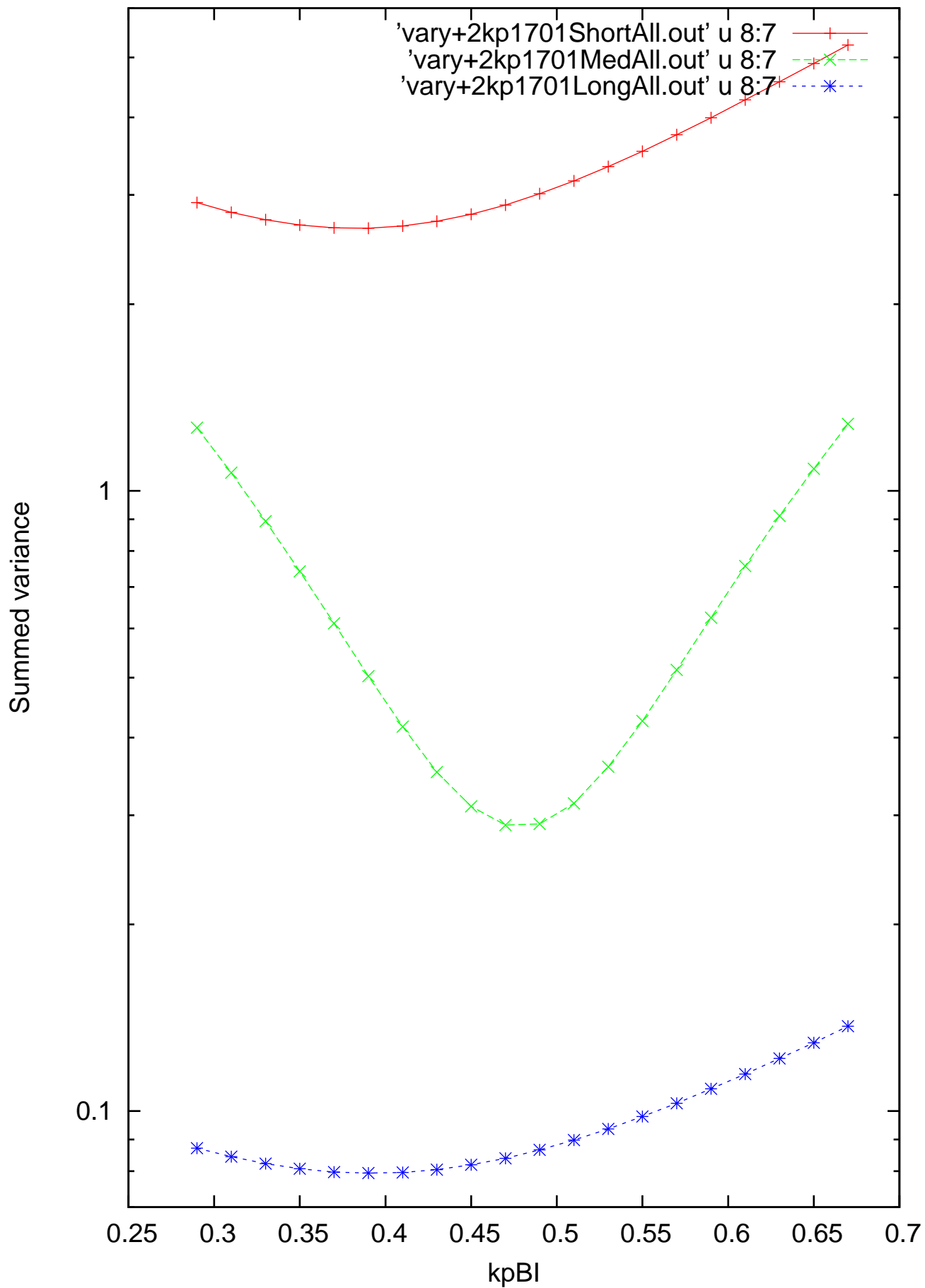
Varying 1701 ED kpBI for m=+2 with ktotBI=1.97
