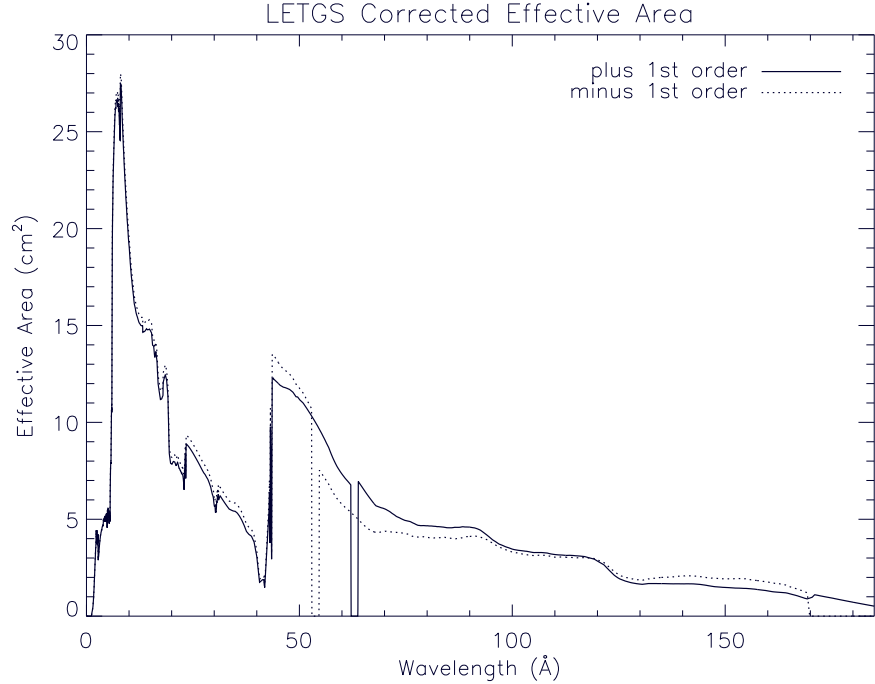
Figure 6. Chandra LETGS effective area, corrected at low energies ( E < 0.277 keV). The solid line is the positive 1st order and the dotted line is the negative 1st order. Dropouts to zero are caused by the plate gaps. Positive and negative order gaps occur at different wavelengths due to displacement of HRC-S center from telescope center.
