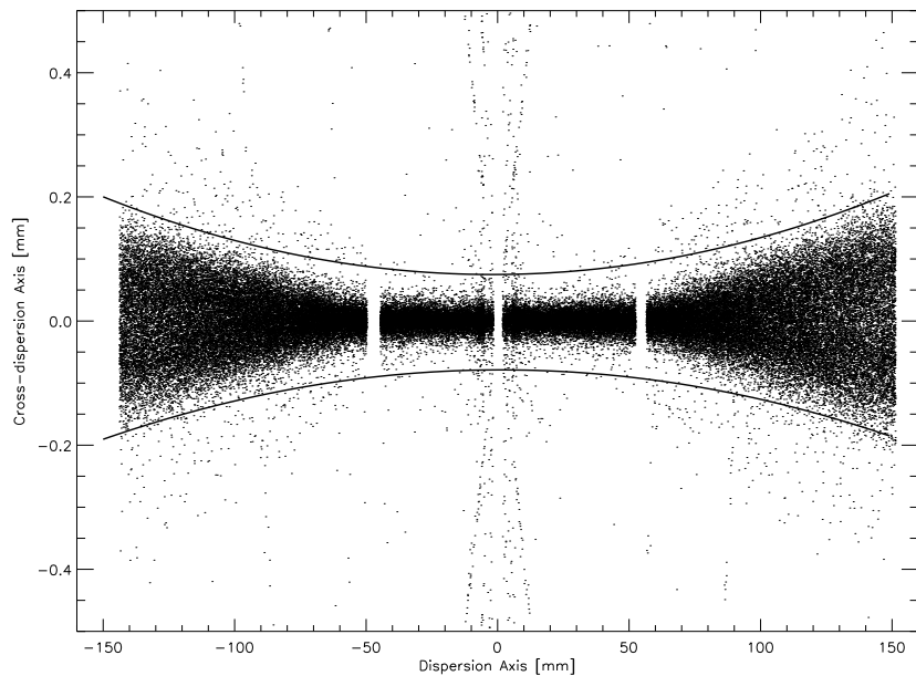
Figure 3. A simulation of a flat spectrum designed to illustrate the broadening of the LETGS profile in the cross-dispersion direction, and the effectiveness of the optimized parabolic spectral extraction region.
