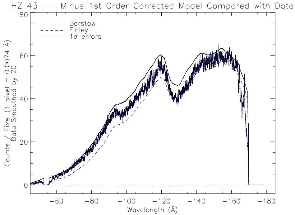
Figure 8. Comparison of two different model-predicted spectra for HZ 43 with the LETGS observed spectrum. Both models show good overall agreement with the data to \approx 10\% . Positive and negative orders plotted separately.
