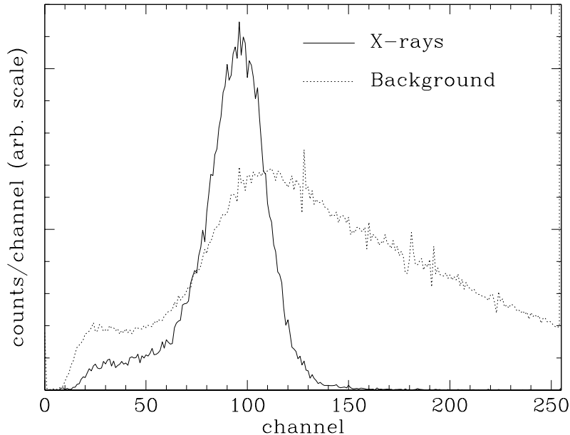
Figure 1. Pulse height spectra of X-rays and background. X-ray spectrum is a sum taken from detector regions ( 128 \times 128 pixels in size) where the mean pha value = 90 \pm 1 . The contribution from background, which is less than 4%, has been subtracted. Background spectrum is taken from a larger area. Channel 255, which contains roughly 25% of the background events, has been truncated for display purposes.
