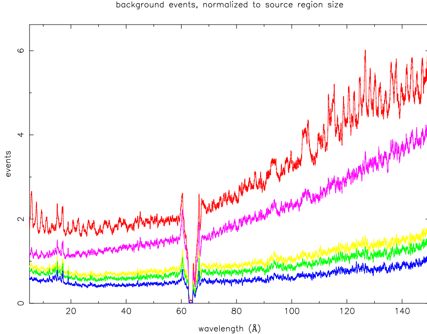
Figure 2. The LETG+HRC-S background spectrum for an observation of Capella using an optimized parabolic spectral extraction window and filtered by pulse height to different levels of X-ray loss (see text). The curves from the top down correspond to: no filtering; pha=255 events removed with 0% X-ray event loss; filtering with 2% X-ray loss; 5% X-ray loss; and 15% X-ray loss. The units of the y axis are total events/bin with a bin size of one pixel ( 6.43 \mu\text{m} , or .0074 \text{ \AA} ). Exposure time was 85 ksec.
