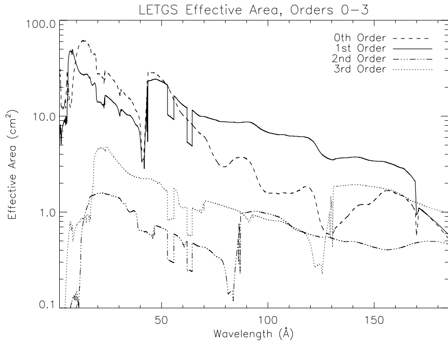
Figure 10. Chandra LETGS effective area for 0th order on-axis (dashed curve), 1st order dispersed (solid curve), 2nd order (dash-dot-dot-dot curve), and 3rd order (dotted curve). Dropouts are caused by the plate gaps. They do not go to zero because the positive and negative order gaps occur at different wavelengths due to the displacement HRC-S center from telescope center.
