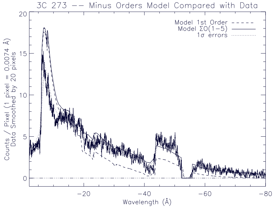
Figure 9. Comparison of the 1st order model-predicted spectrum (dashed curve) and the \Sigma O(1-5) model-predicted spectrum (solid curve) for 3C 273 with the LETGS observed spectrum. The summed orders model shows good agreement with the observed spectrum over the energy range 0.2–0.8 keV, illustrating the significance of high order contributions. Positive and negative orders plotted separately.
