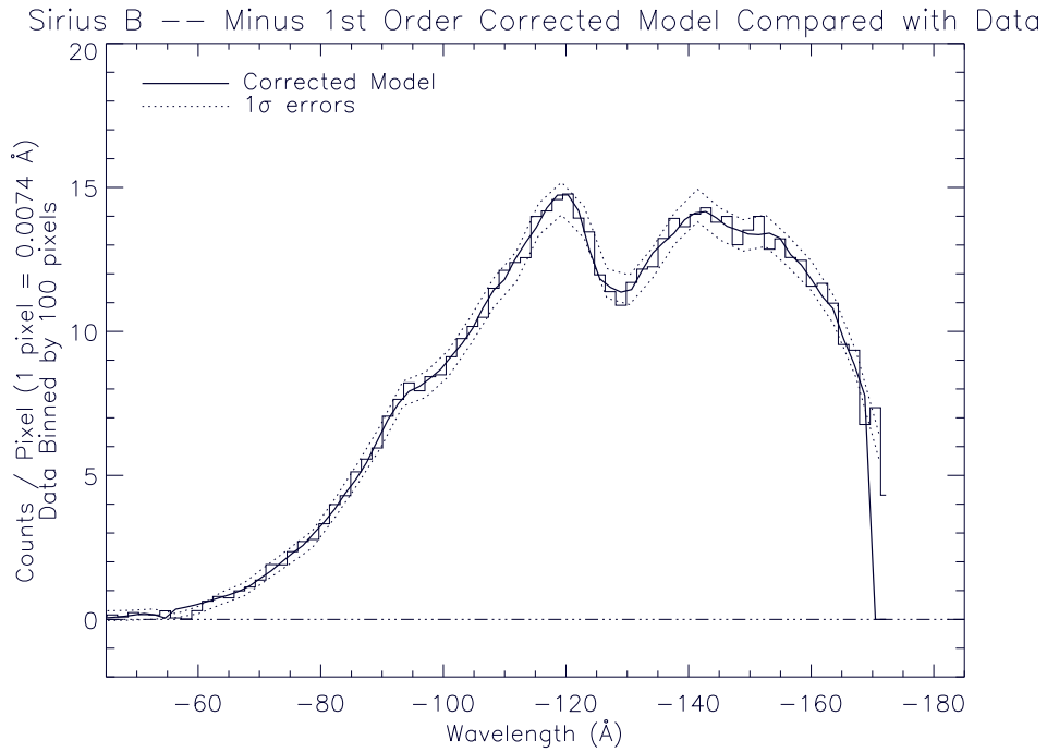
Figure 7. Re-Comparison of the “corrected” model-predicted spectrum for Sirius B with the LETGS observed spectrum. Positive and negative orders plotted separately.
