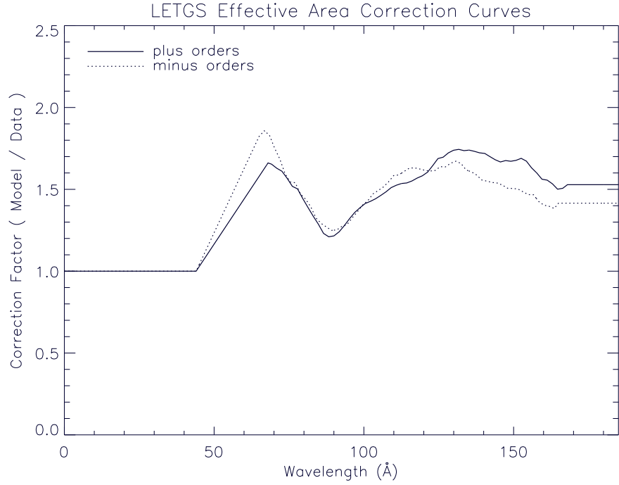
Figure 5. Chandra LETGS effective area correction curves derived from model-to-data comparison with Sirius B. Solid line is the correction to the positive orders and the dotted line is the correction to the negative orders.
