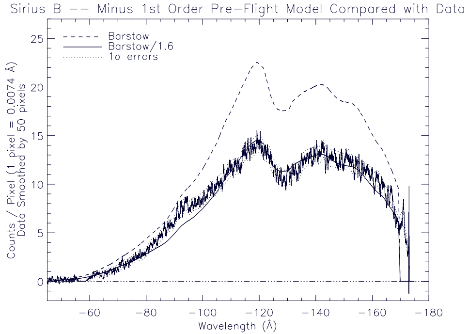
Figure 4. Comparison of the pre-flight model-predicted spectrum for Sirius B with the LETGS observed spectrum indicate that the pre-flight low energy HRC-S QE is overestimated by an average factor of about 1.6. Dashed line is the model, solid line is the model/1.6, and dotted lines are the 1\sigma statistical errors on the data. Positive and negative orders plotted separately.
