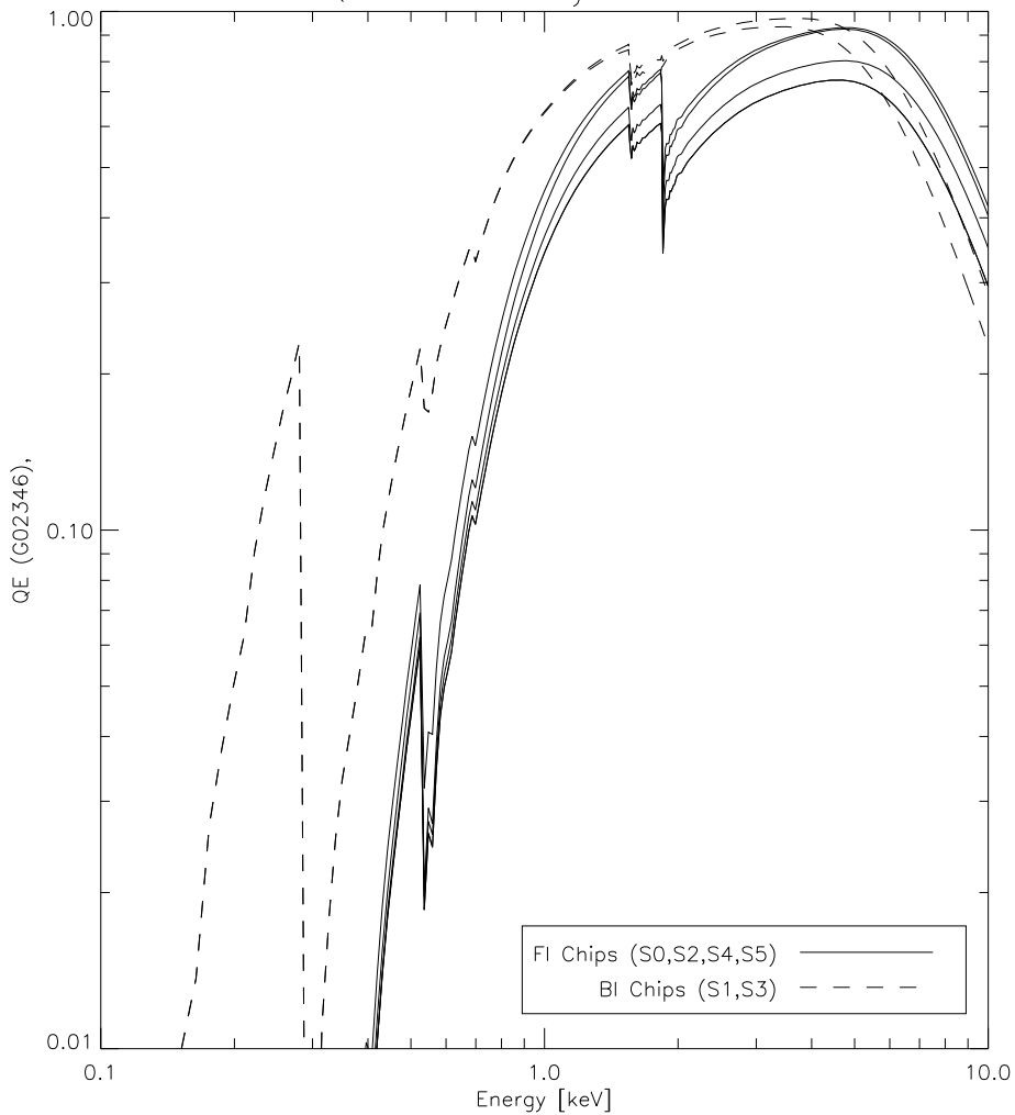
Quantum Efficiency * filt. trans.
