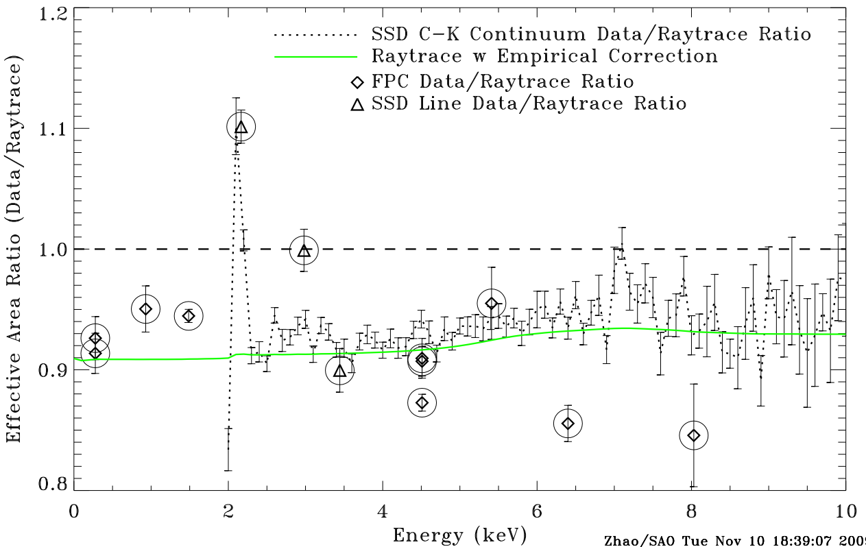
XRCF HRMA Effective Area Ratio within 2 mm, CH2: 28,18,20,27Å
