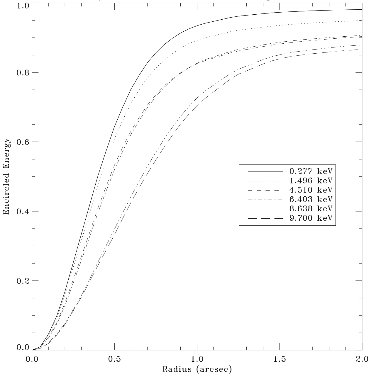
HRMA/ACIS-S On-axis PSF with Aspect Error
