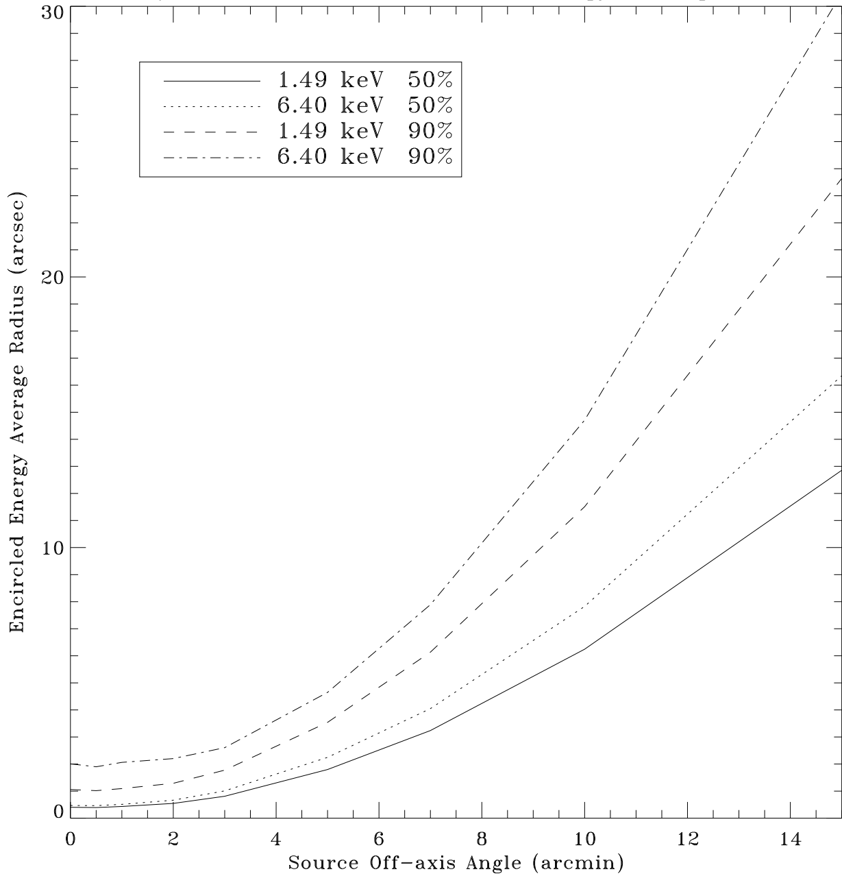
HRMA/HRC-I Off-axis Encircled Energy Average Radius
