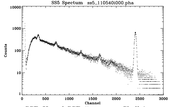
SSD-X and SSD-5 spectra: Shell 3.
