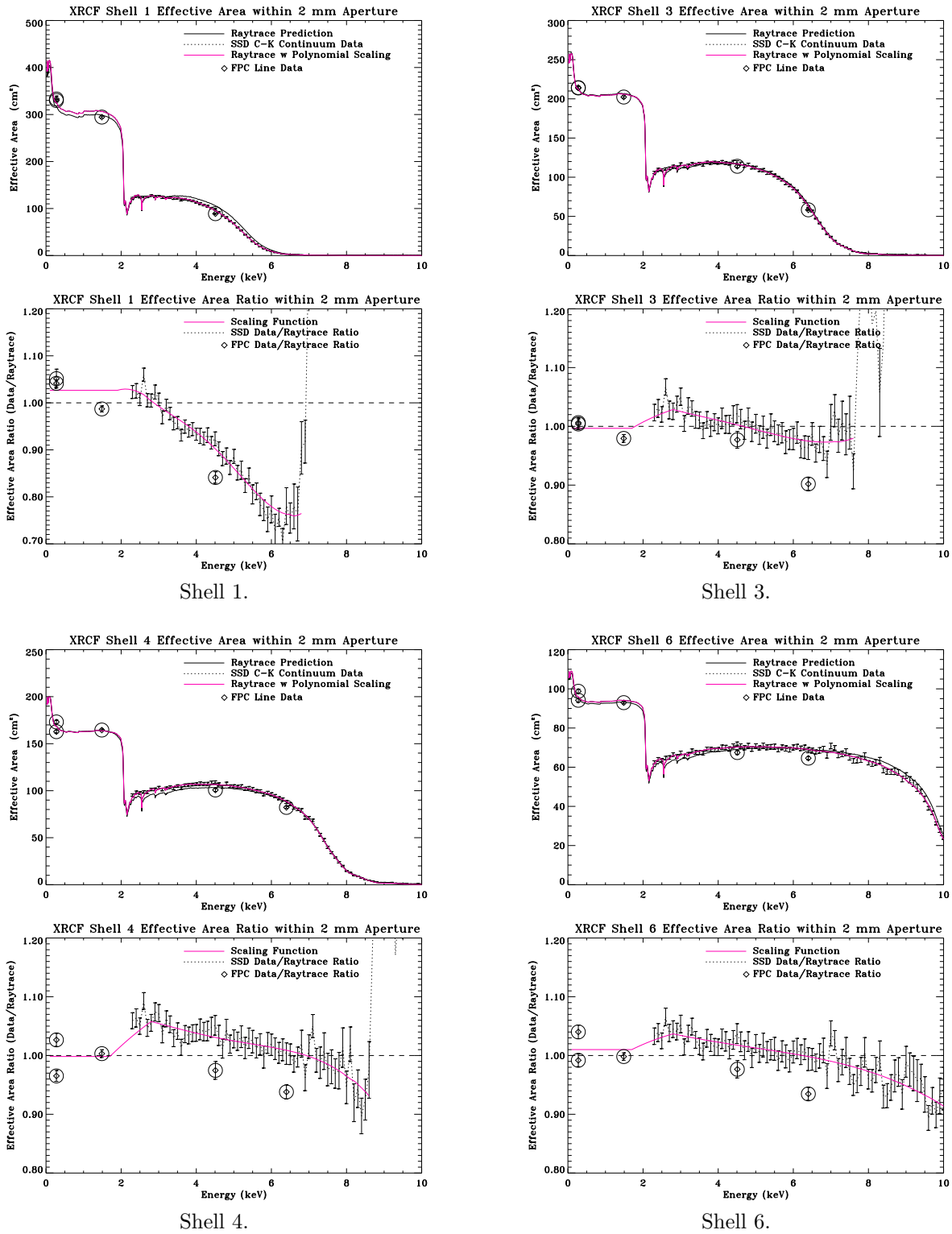
Figure 5. Calibration data vs. raytrace prediction. Top panel of each quadrant plot shows the XRCF effective area within 2 mm aperture. Bottom panel shows the effective area ratio of data/raytrace.
