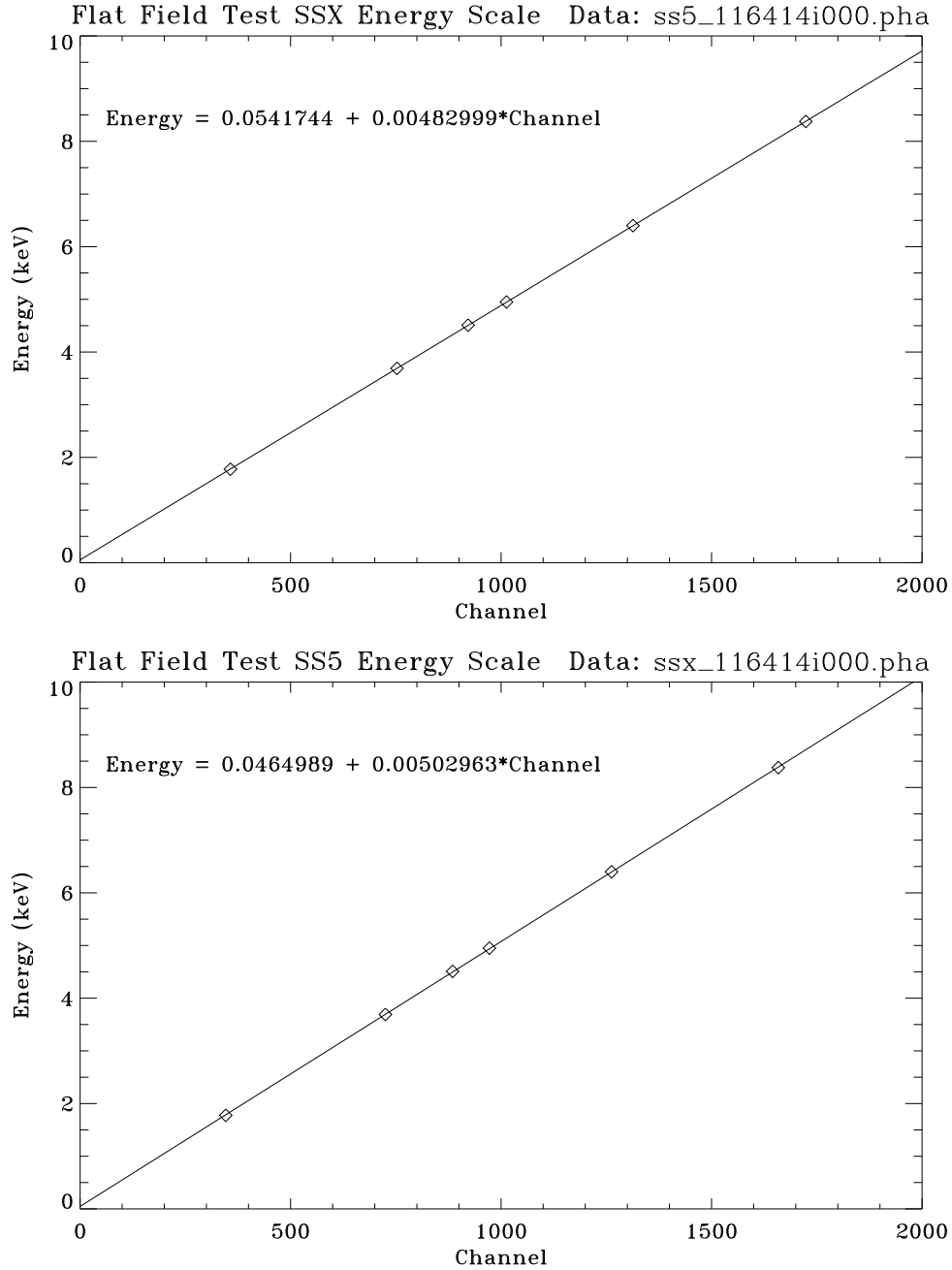
Figure 3. SSD-X and SSD-5 energy scales for the flat field test, fitted with six X-ray line energies.
