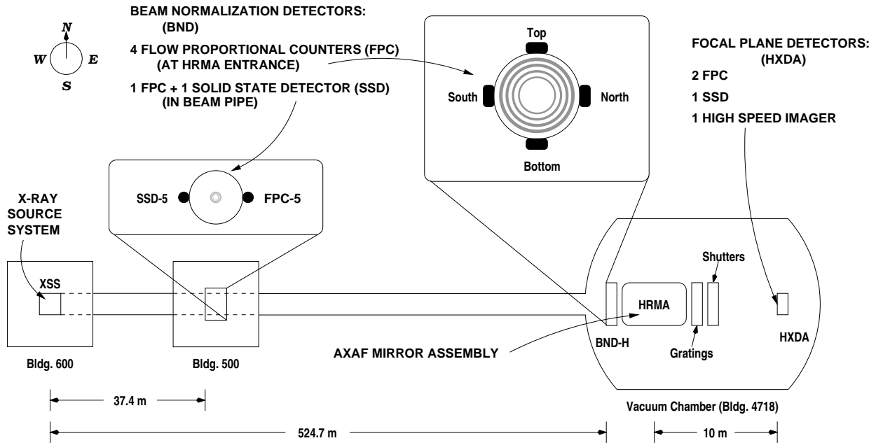
Figure 1. HRMA Calibration configuration at the XRCF.
