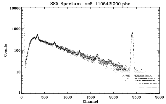
SSD-X and SSD-5 spectra: Shell 6.
