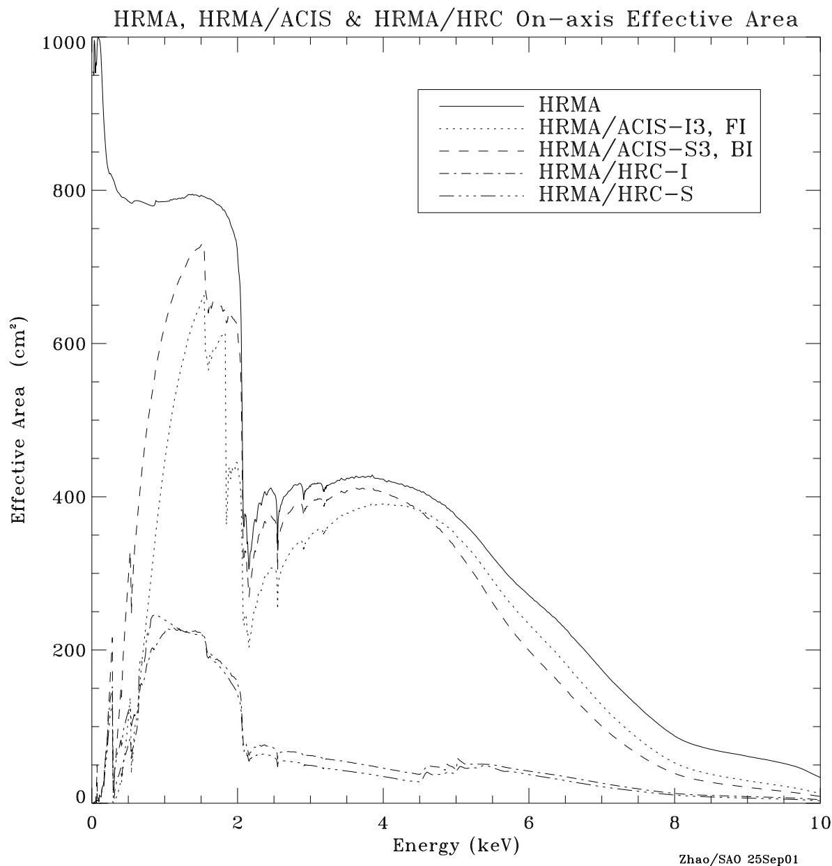
Figure 8. The HRMA, HRMA/ACIS and HRMA/HRC effective areas versus X-ray energy in linear scale. The structure near 2 keV is due to the iridium M-edge. The HRMA effective area is calculated by the raytrace simulation based on the HRMA model and scaled by the XRCF calibration data. The HRMA/ACIS effective areas are the products of HRMA effective area and the Quantum Efficiency (QE) of ACIS-I3 (front illuminated) or ACIS-S3 (back illuminated). The HRMA/HRC effective areas are the products of HRMA effective area and the QE of HRC-I or HRC-S at their aimpoints, including the effect of UV/Ion Shields (UVIS).
