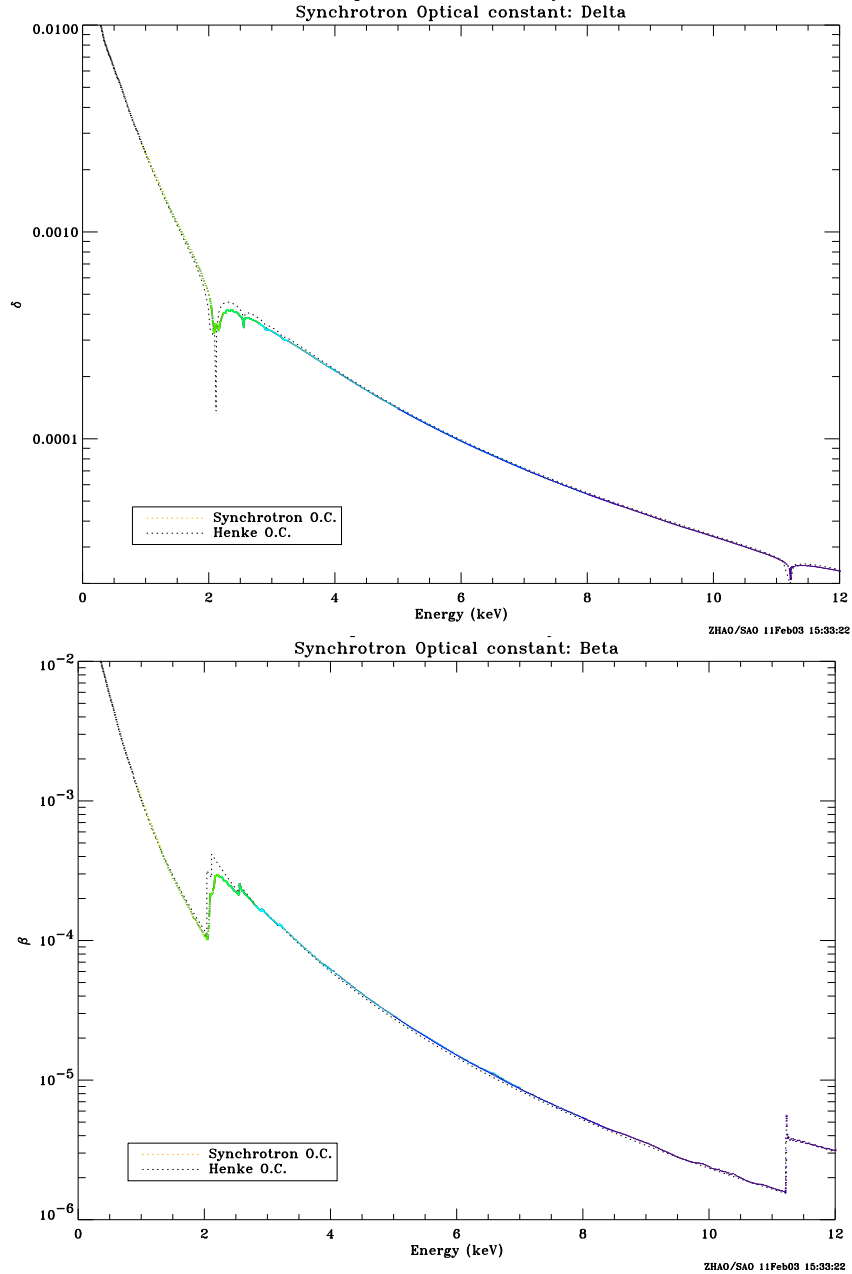
Figure 4. Ir optical constants from the BNL synchrotron measurements.
