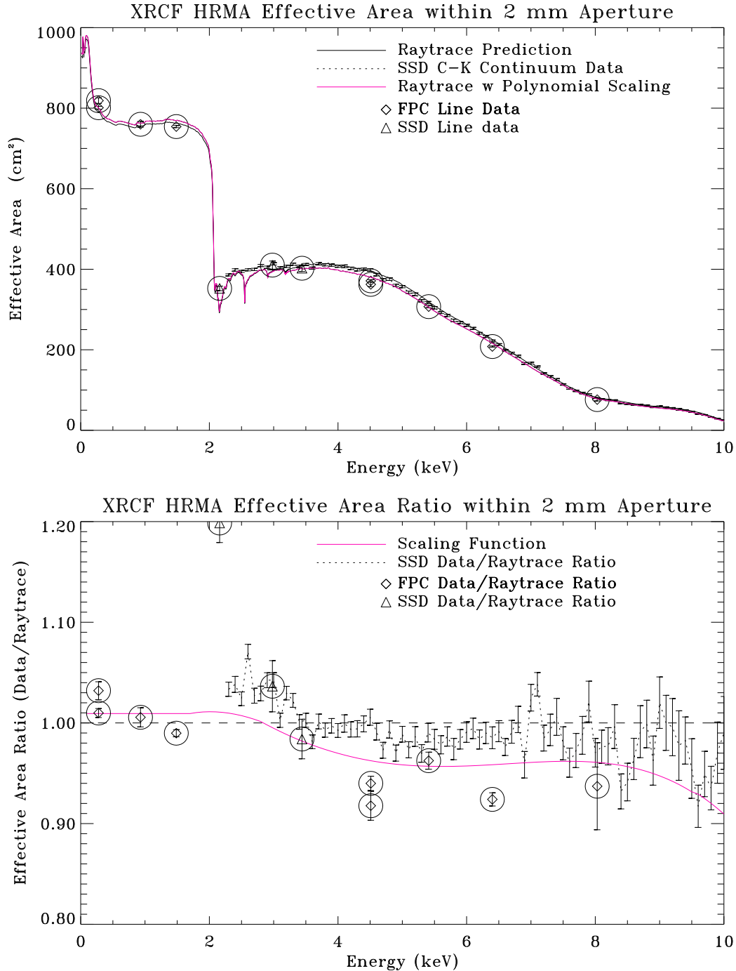
Figure 7. The HRMA effective area measured at the XRCF. In the upper panel: the solid line is the raytrace simulation of the HRMA effective area within a 2 mm diameter aperture at the focus; the dashed line with error bars shows the SSD data with a C-K continuum source; the diamonds and triangles show the FPC and SSD data with spectral line sources. The lower panel shows deviation of data from the raytrace: the dashed line with error bars is the ratio of SSD C-K continuum data vs. the raytrace; the diamonds and triangles show the ratio of FPC and SSD spectral line data vs. the raytrace; the solid line is a polynomial function, which gives equal weight to the deviations of the continuum and line measurements, for scaling the raytrace simulation to provide the predicted HRMA effective area.
