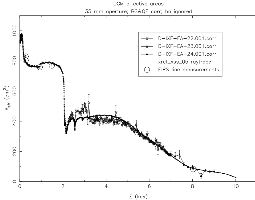
Figure 10. DCM Effective Area Measurements. The results are comparable to SSD continuum and FPC line measurements. The Ir edge structure in the 2-3 keV range is resolved. the jump near 3 keV is almost certainly the Ar edge in the FPC response.
