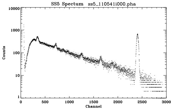
SSD-X and SSD-5 spectra: Shell 4.
