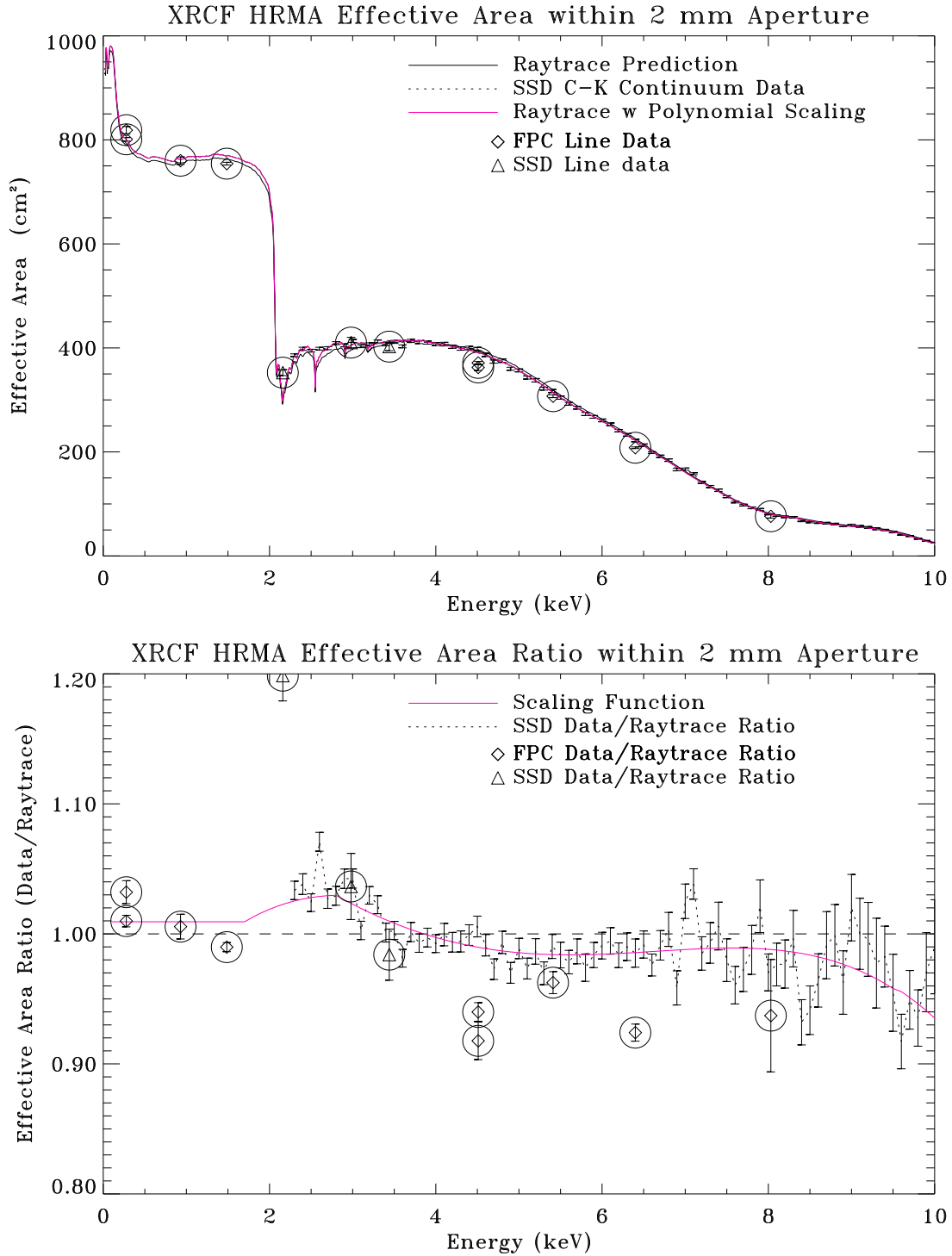
Figure 6. Calibration data vs. raytrace prediction. Top panel shows the XRCF HRMA effective area within 2 mm aperture. Bottom panel shows the effective area ratio of data/raytrace.
