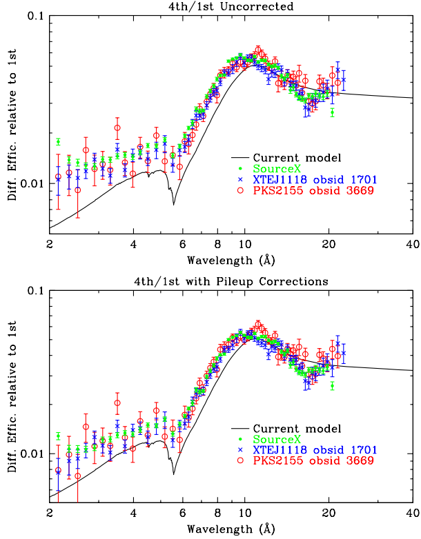
Figure 7. Ratio of 4th and 1st order efficiencies. Longward of \sim 15 Å, ROI analysis cannot adequately separate the 4th- and 3rd-order energy-spectrum peaks.
