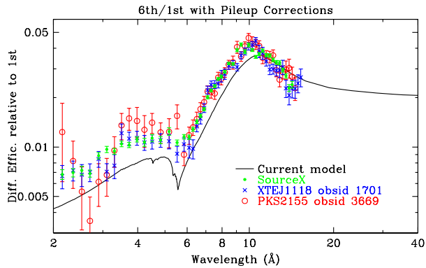
Figure 9. Ratio of 6th and 1st order efficiencies.
