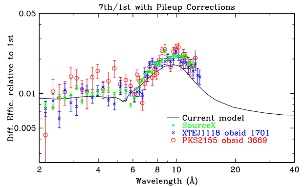
Figure 10. Ratio of 7th and 1st-order efficiencies.
