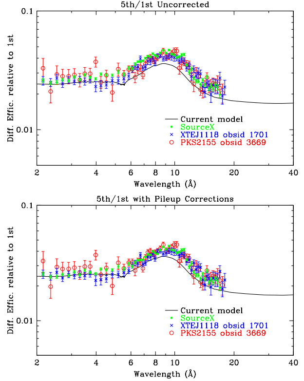
Figure 8. Ratio of 5th and 1st-order efficiencies. Current model appears to be \sim 15\% low at most wavelengths, but the overall agreement in shape is good.
