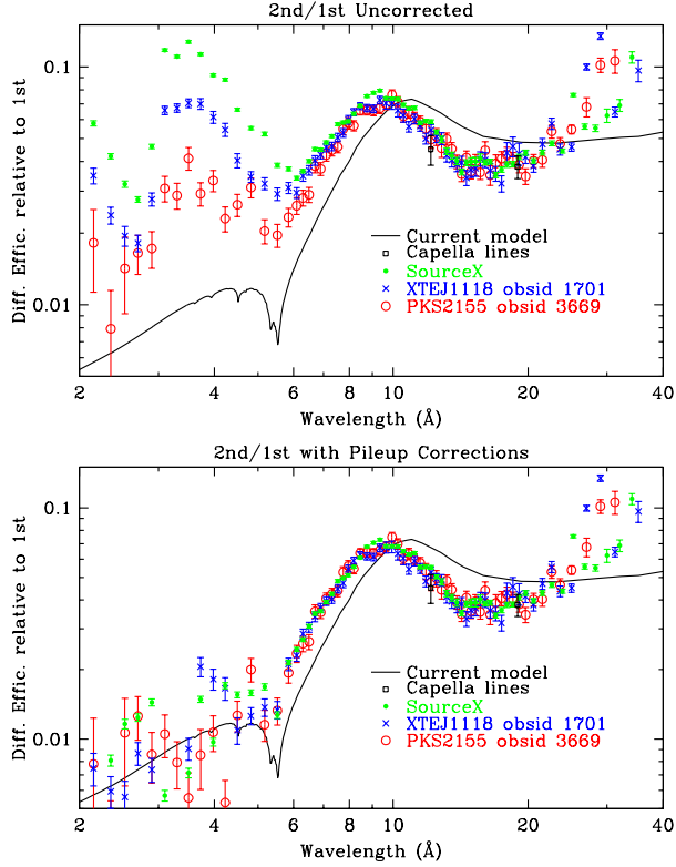
Figure 5. Ratio of 2nd and 1st-order efficiencies, showing results without pile-up corrections (top panel) and with corrections (bottom). Pile-up of 1st-order events is obvious below 6 Å. Points beyond \sim 20 Å are spurious; the 2nd-order energy-spectrum peak cannot be cleanly separated using ROI analysis from the stronger 3rd-order peak.
