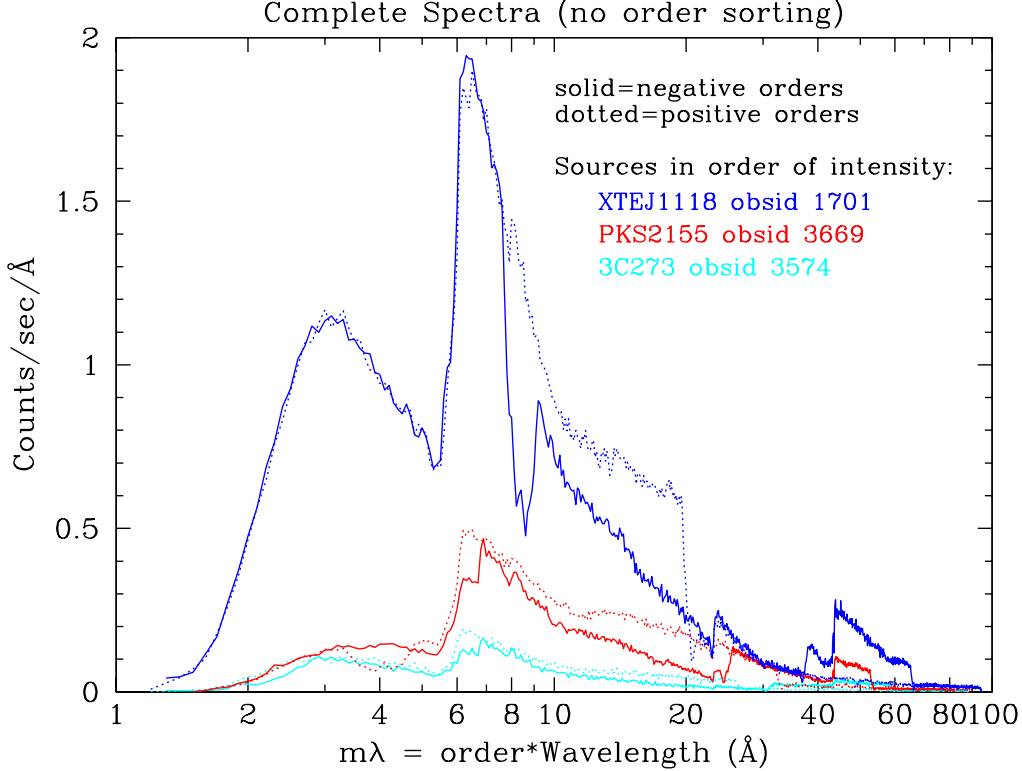
Figure 2. Spectra used in this analysis, showing widely varying rates. The SourceX spectrum is not shown, as the data are still proprietary, but the source is more than 50% brighter than XTEJ1118. Analysis results from 3C 273 are not shown in subsequent figures, as the data points have very large statistical error bars.
