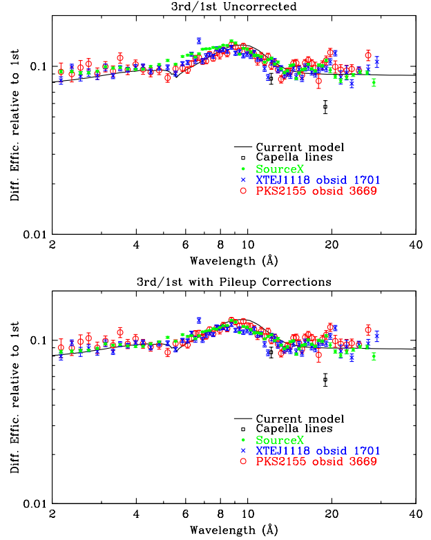
Figure 6. Ratio of 3rd and 1st-order grating efficiencies. Agreement with the current model is very good, but can be improved by roughly 10% at wavelengths beyond \sim 8 Å. Beyond the “bump”, data from line sources collected with the HRC-S will be important in calibrating the longer-wavelength efficiencies.
