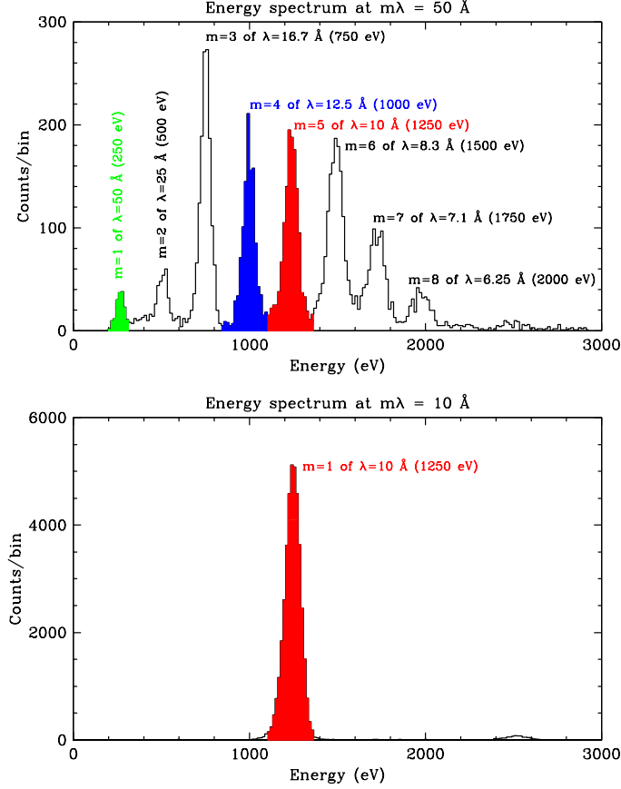
Figure 4. Example energy spectra. Top panel is for the wavelength range m\lambda = 49.0 to 50.5 Å. Colored shading shows which peaks are used to determine the pile-up-corrected number of counts in 5th order of 10 Å. The total number of counts in the entire spectrum is also used in pile-up calculations (see Eqs. 3 and 4). In this example, pile-up corrections are negligible. For comparison, the 1st order spectrum of 10 Å (used in calculation of the 10 -Å 5th/1st efficiency ratio) is shown in the bottom panel.
