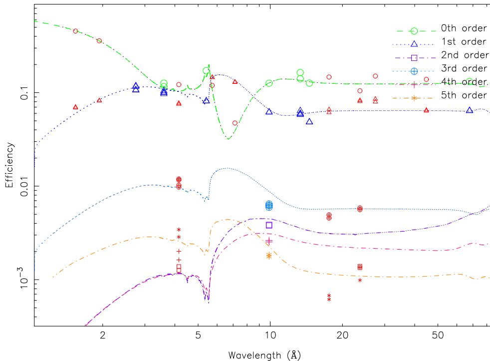
Figure 1. LETG efficiencies from ground calibration at XRCF, using Electron Impact Point Source data. Smaller red symbols mark cases where model HRMA effective area predictions were used in lieu of unavailable grating-out measurements. Higher-order calibration was sparse, but seems to indicate some disagreements with current calibration model predictions (continuous lines).
