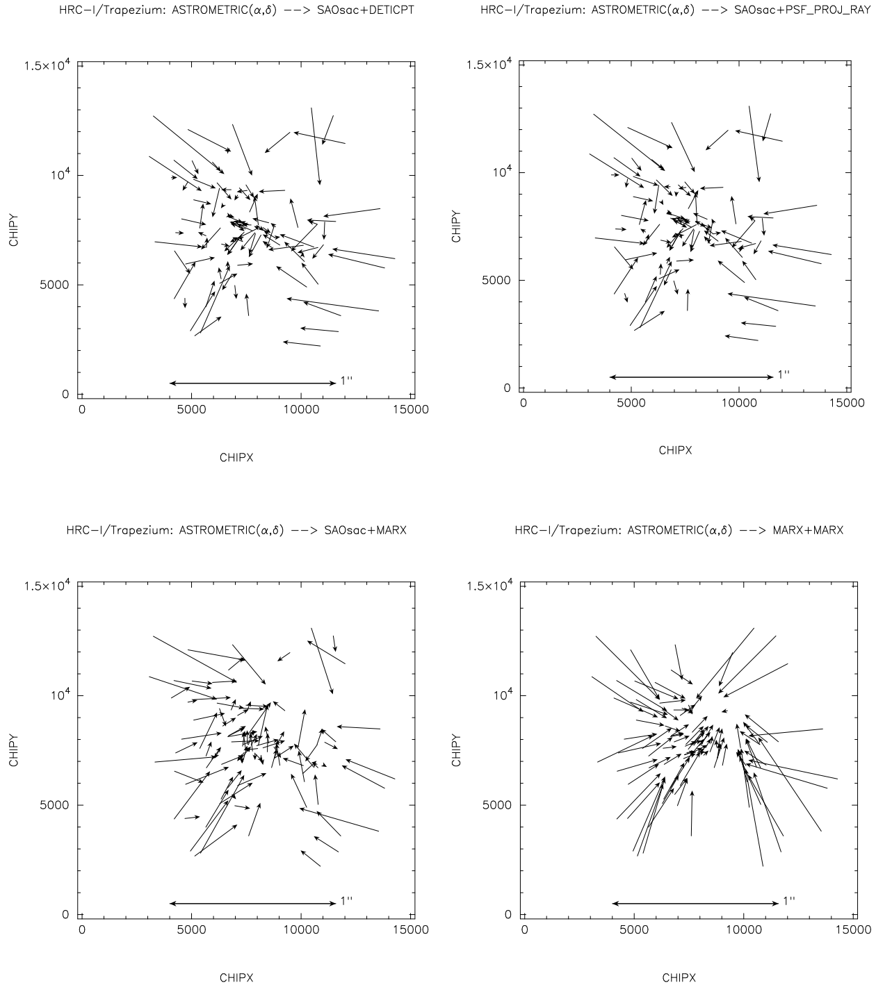
Figure 5. ONC: Positional shifts from CHIP positions determined by dmcoords based on the optical astrometry and the nominal pointing, to where the models predict they would be imaged. The scaling convention follows that in Fig. 3.
