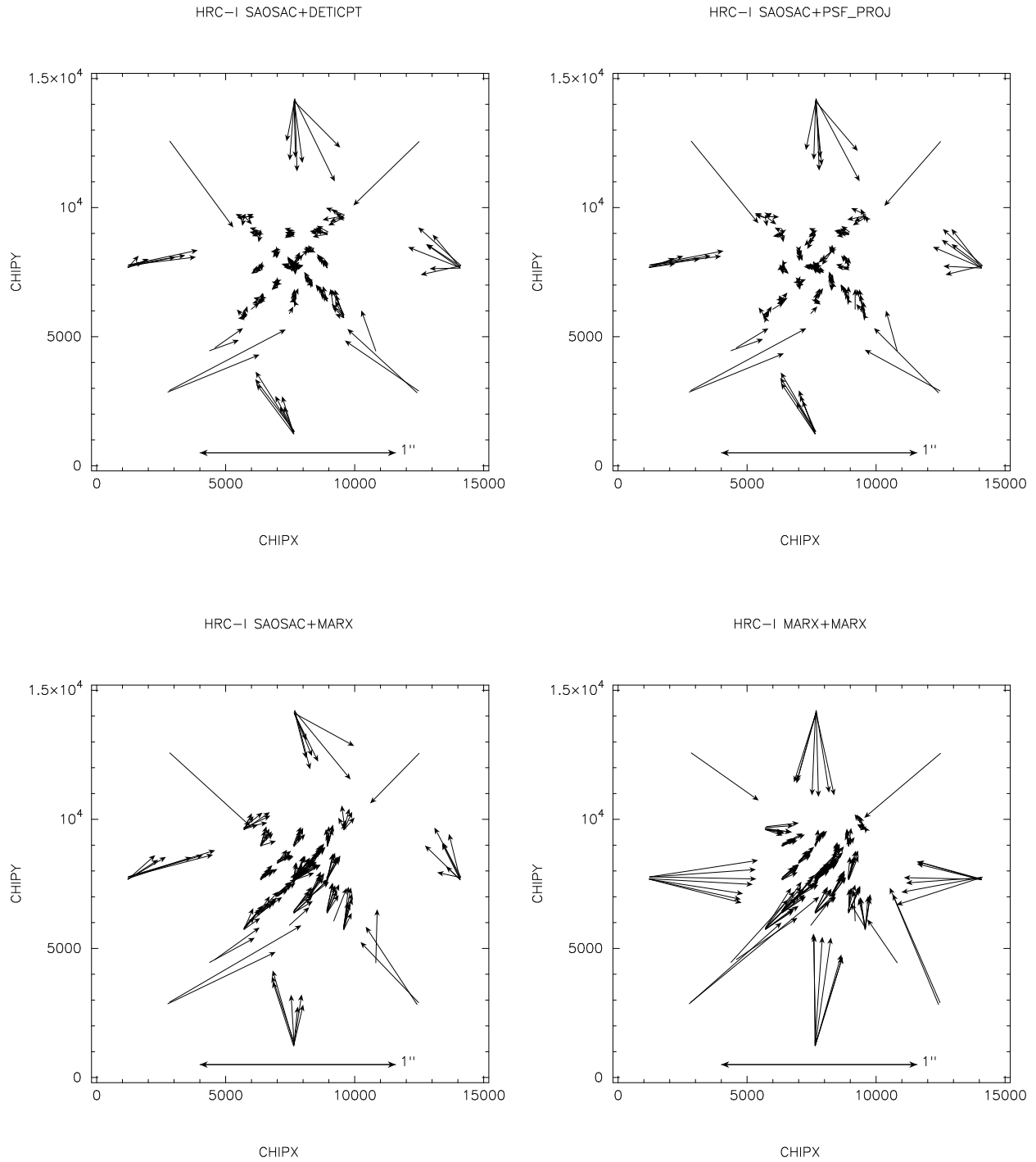
Figure 3. Individual bright point source observations: vector diagrams representing the shift from centroids of the observed detections to centroids of the simulated rays. Positional offsets are scaled by a factor of 1000 to exaggerate the deviations. The arrow at the bottom denotes shifts of 1'' ( \sim 7.5 HRC pixels) in this scaling convention. Quantitative analysis of these offsets is shown in Table 1.
