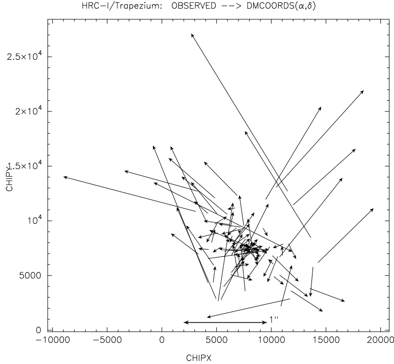
Figure 6. ONC: Positional shifts from observed centroids to the CHIP positions determined by dmcoords based on the optical astrometry and the nominal pointing of the telescope. The scaling convention follows that in Fig. 3.
