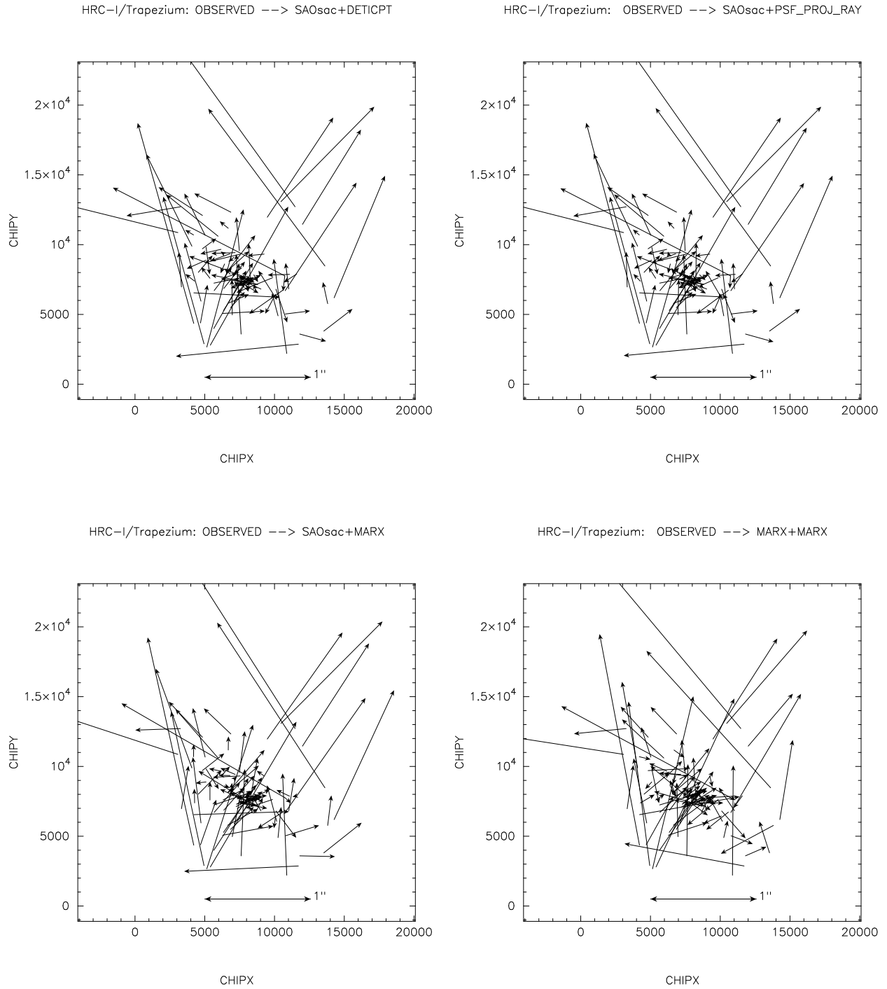
Figure 4. ONC: Positional shifts from where the sources were observed in CHIP coordinates to where the simulations placed them on the detector. The scaling convention follows that in Fig. 3.
