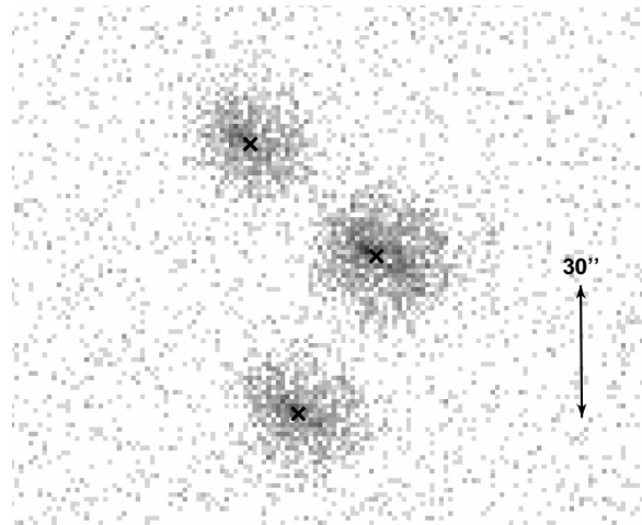
Figure 1. LEFT: The Orion Nebular Cluster on HRC-I, in SKY coordinates, as determined by standard pipeline processing. RIGHT: ONC on HRC-I in CHIP coordinates, after telescope dither is manually removed.
