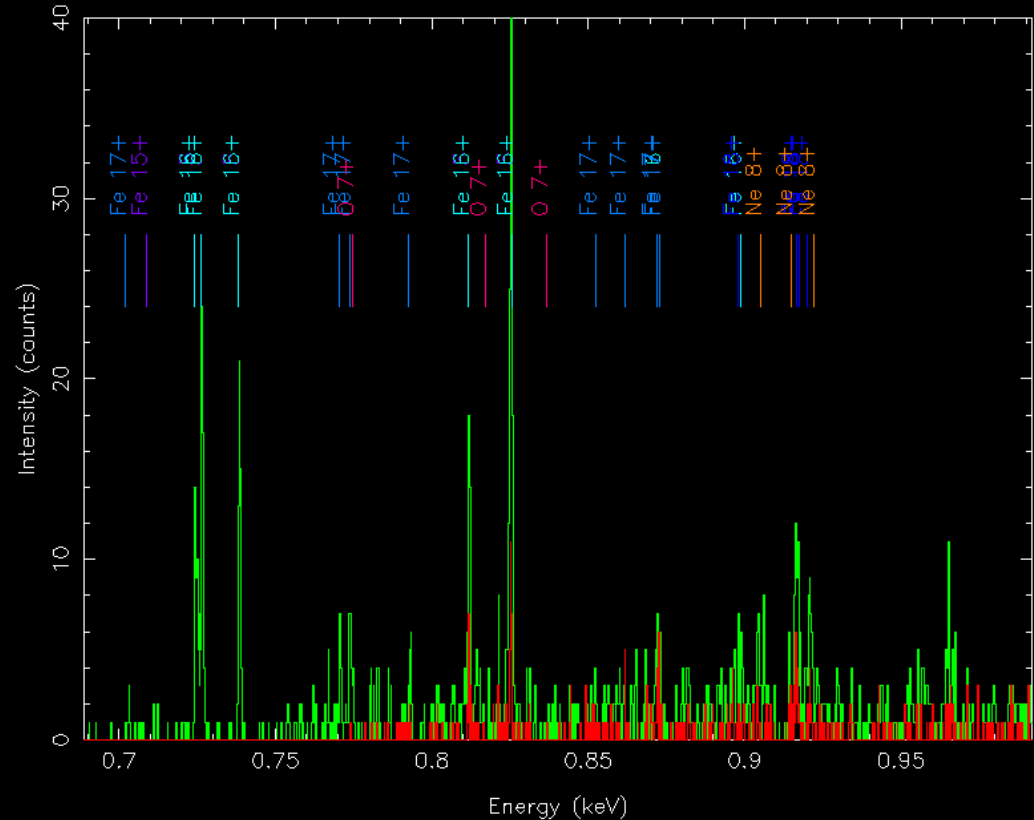
HETGS Capella First-light, OBSID 1098: Fe region
