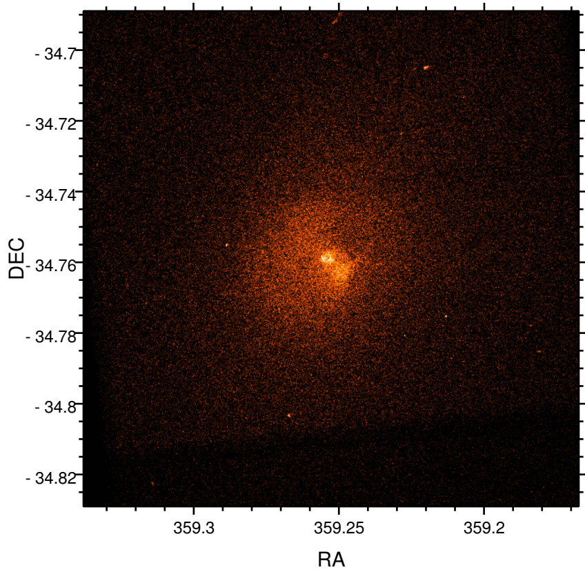
ABELL 4059
