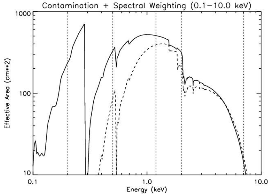
Fig. 3: This is a plot of the product of the effective area of the telescope with quantum efficiency of the detector times a spectral weighting function (see text). The solid line is the back illuminated chip (S3) and the dashed line is the front illuminated chip (I3). The dotted lines are the energy boundaries of the CSC bands.
