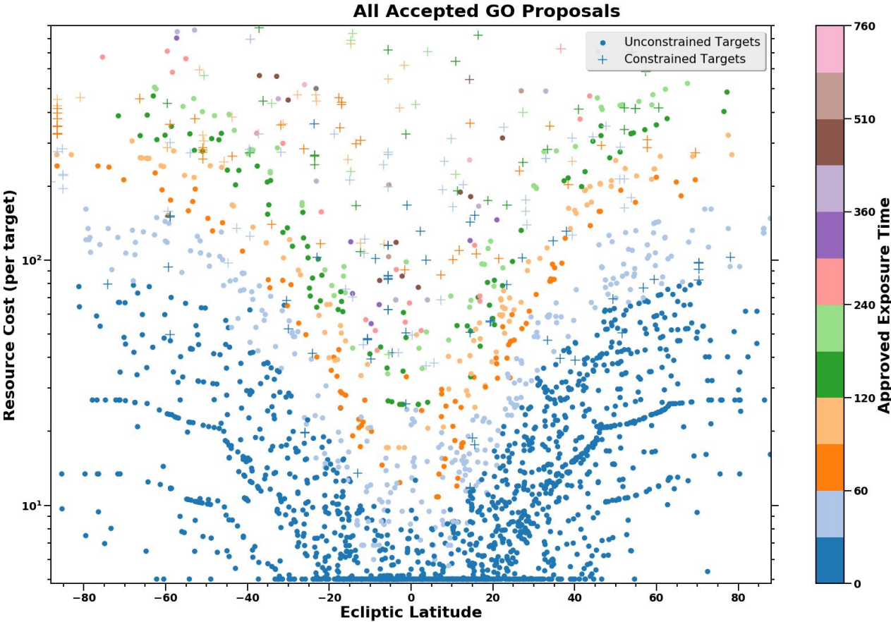
Figure 1: Plot of Resource Cost (RC) values for observing programs from Chandra Cycles 14-22, calculated using RC formulation for Cycle 23. Circles correspond to observations without constraints, for which RC values are dominated by the ecliptic latitude (X-axis) and exposure time (color bar at right). Crosses correspond to targets with observing constraints, for which the nature and difficulty of the constraint is compounded with the values associated with the sky position and exposure time. The plot is truncated at RC values of 900, but larger values can result for highly-constrained, long observations.
