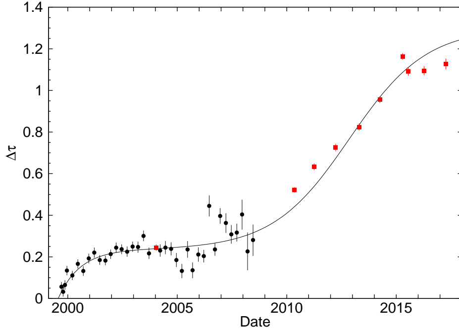
Figure 6.8: The difference between the optical depth at 0.66 keV measured near the center of the ACIS-S chip S3 and that measured near the readout at the edge of the same chip is shown against time. Black circles are measurements made using the ECS data and red squares are made from observations of the galaxy cluster Abell 1795. The solid curve is the best-fit relation to the data.
