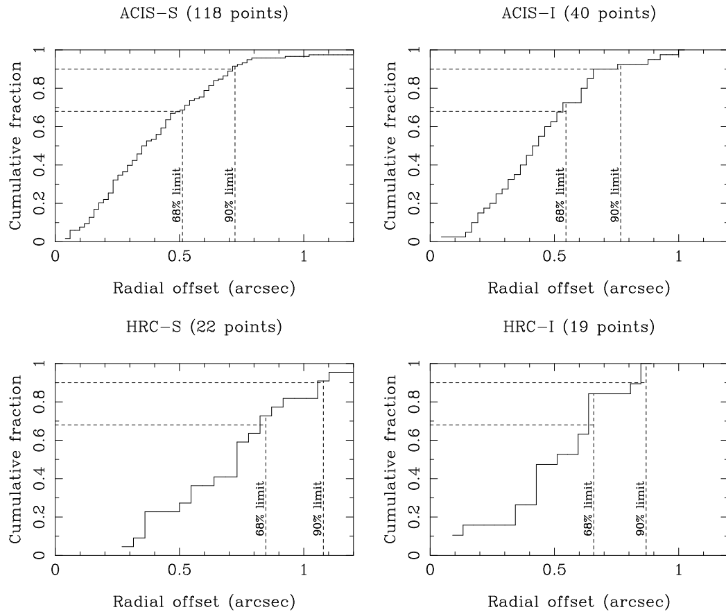
Figure 5.4: Cumulative histogram of celestial accuracy for Chandra X-ray source locations for each SI using observations since Oct-2013. Radial offset is the distance in arcsec between the optical coordinate, typically from the Tycho-2 catalog, and the Chandra position.
