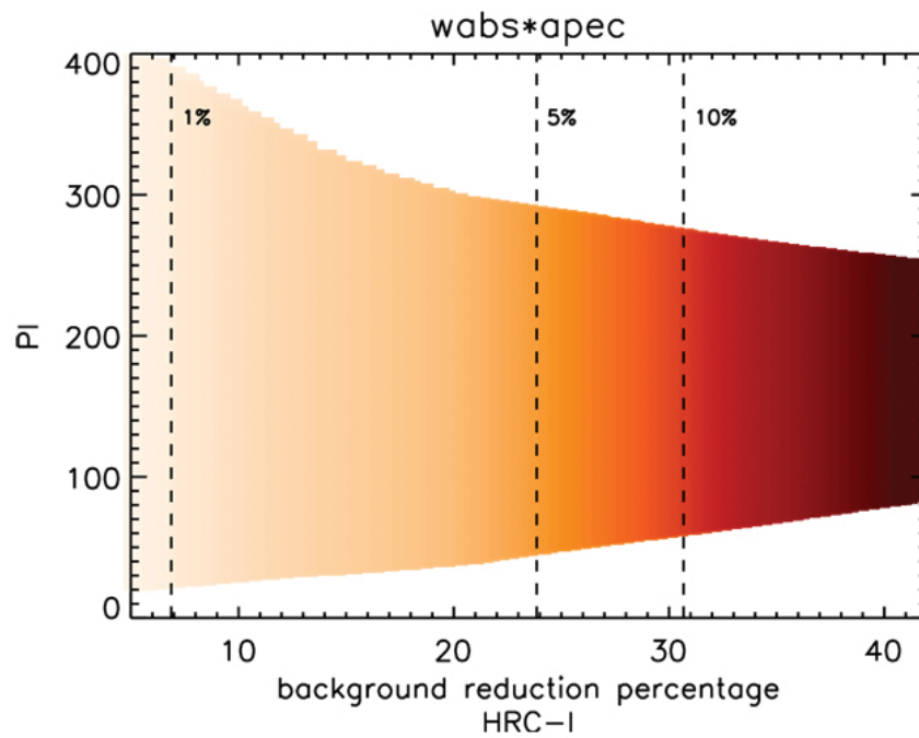
Figure 7.22: As Figure 7.21, but for sources with thermal spectra, for parameter values depicted in Figures 7.10, 7.11.
