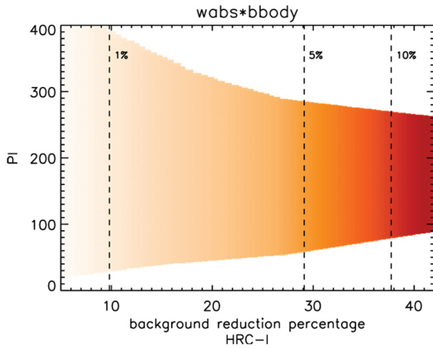
Figure 7.23: As Figure 7.21, but for sources with blackbody spectra, for parameter values depicted in Figure 7.12.
