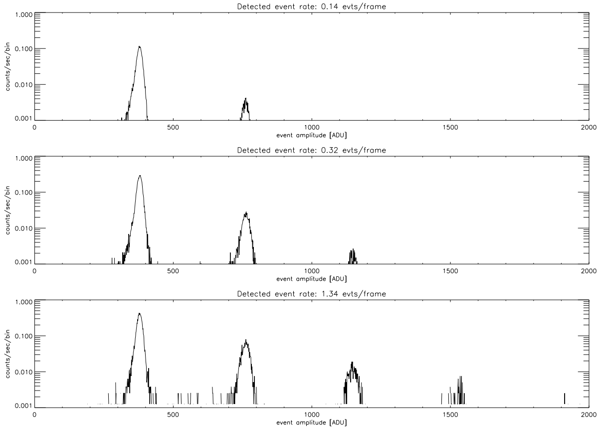
Figure 6.20: The effects of pile-up at 1.49 keV ( \text{Al K}\alpha ) as a function of source intensity. Data were taken during HRMA-ACIS system level calibration at the XRCF. Single-photon events are concentrated near the pulse height corresponding to the \text{Al K}\alpha line ( \sim 380 ADU), and events with 2 or more photons appear at integral multiples of the line energy.
