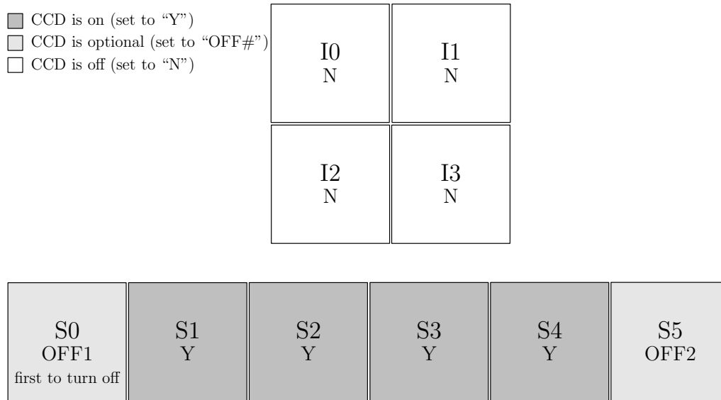
Figure 6.42: ACIS-S spectroscopy, nominal aimpoint (4 Required CCDs, 2 Optional CCDs)
