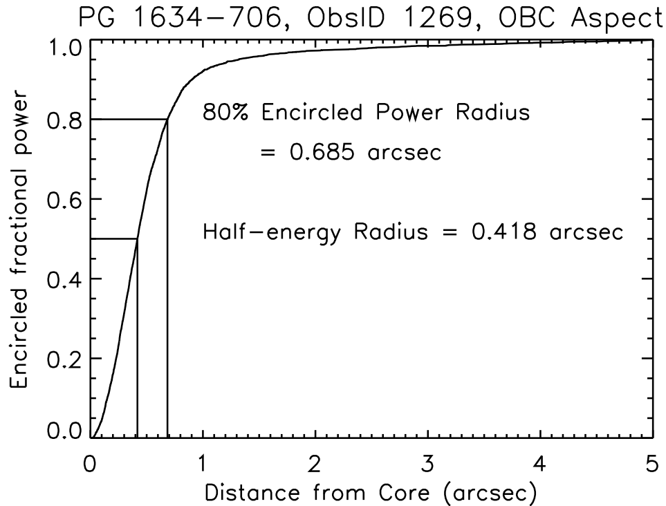
Figure 6.10: The on-orbit encircled broad-band energy versus radius for an ACIS observation of point source PG1634-706 (ObsID 1269). The curve is normalized to unity at a radius of 5 arcsec. We estimate that the statistical uncertainty is 3%, and the systematic uncertainty due to power beyond 5'' is 2%. The effective energy is 1 keV.
