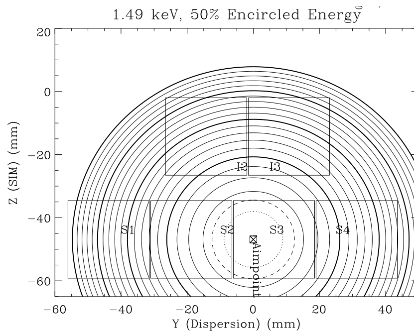
Figure 6.16: Approximate contours of constant 50% encircled energy at 1.49 keV when the ACIS-S aimpoint is selected. The dotted line is 1 arcsec, the dashed line is 1.5 arcsec. The remainder are at 1 arcsec intervals. The thicker solid lines highlight the 5, 10, 15 and 20 arcsec contours.
