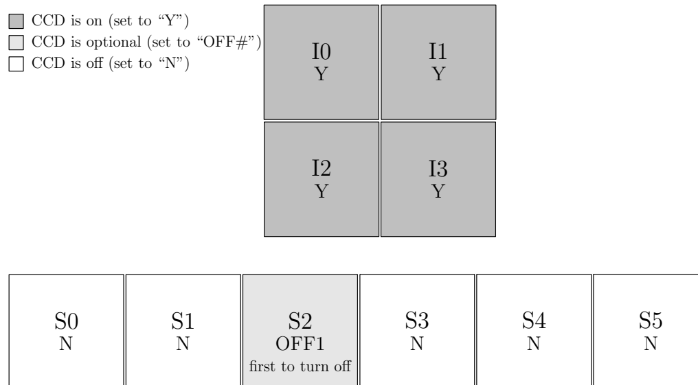
Figure 6.36: ACIS-I imaging, nominal aimpoint (4 Required CCDs, 1 Optional CCD)
