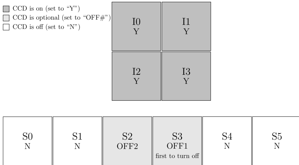
Figure 6.38: ACIS-I imaging, nominal aimpoint (4 Required CCDs, 2 Optional CCDs)
