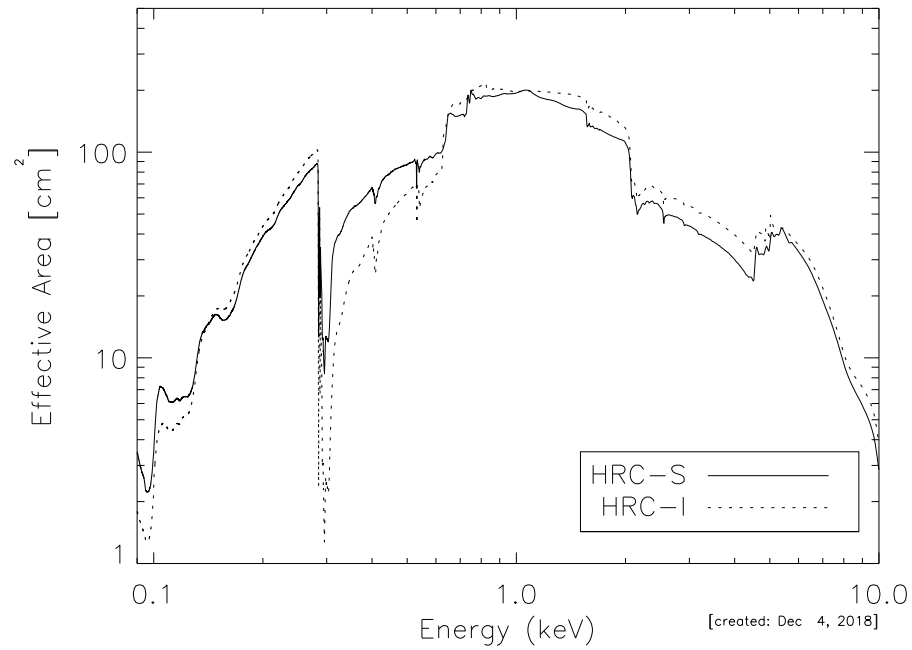
Figure 7.17: The effective area of the HRMA/HRC-I (dashed line) and the central segment of the HRMA/HRC-S in imaging mode (solid line) integrated over the full PSF. Absorption edges are due to the iridium coating on the mirrors, the CsI MCP coating, and the polyimide/Al of the UVIS.
