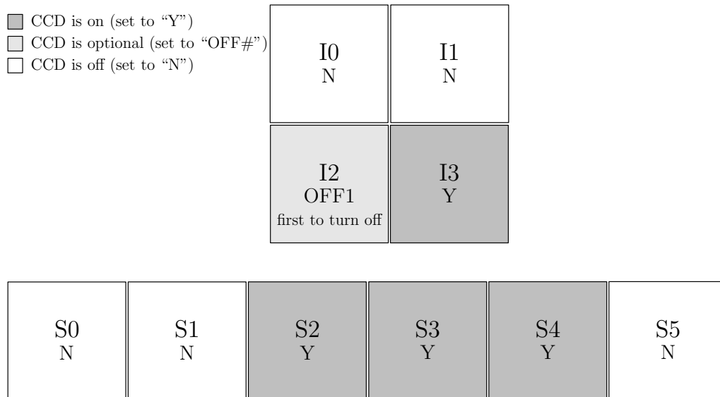
Figure 6.39: ACIS-S imaging, nominal aimpoint (4 Required CCDs, 1 Optional CCD)
