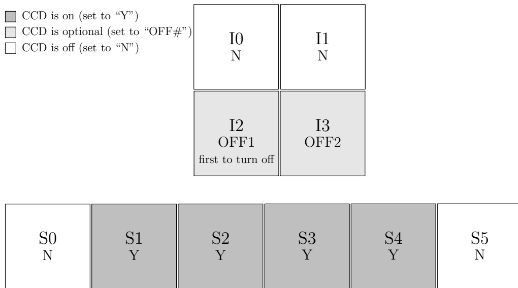
Figure 6.41: ACIS-S imaging, nominal aimpoint (4 Required CCDs, 2 Optional CCDs)
