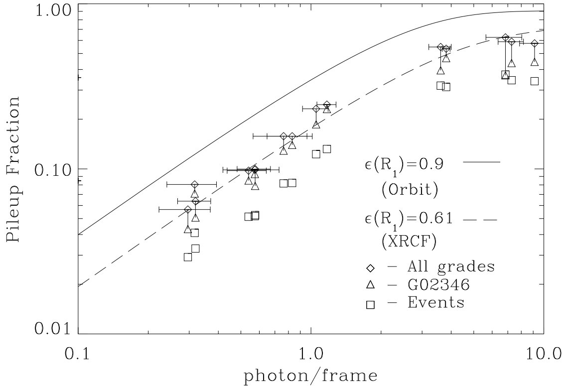
Figure 6.22: The pile-up fraction as a function of the the counting rate (in the absence of pile-up in units of photons/frame). The solid line is for on-orbit, the dashed line and the data points are for, and from, ground-based data respectively. The difference between the ground and flight functions are a consequence of the improved PSF on-orbit, where gravitational effects are negligible – see Chapter 4. Note that when pile-up occurs there are two or more photons for each event, so the fraction of events with pile-up is always less than the fraction of photons with pile-up.
