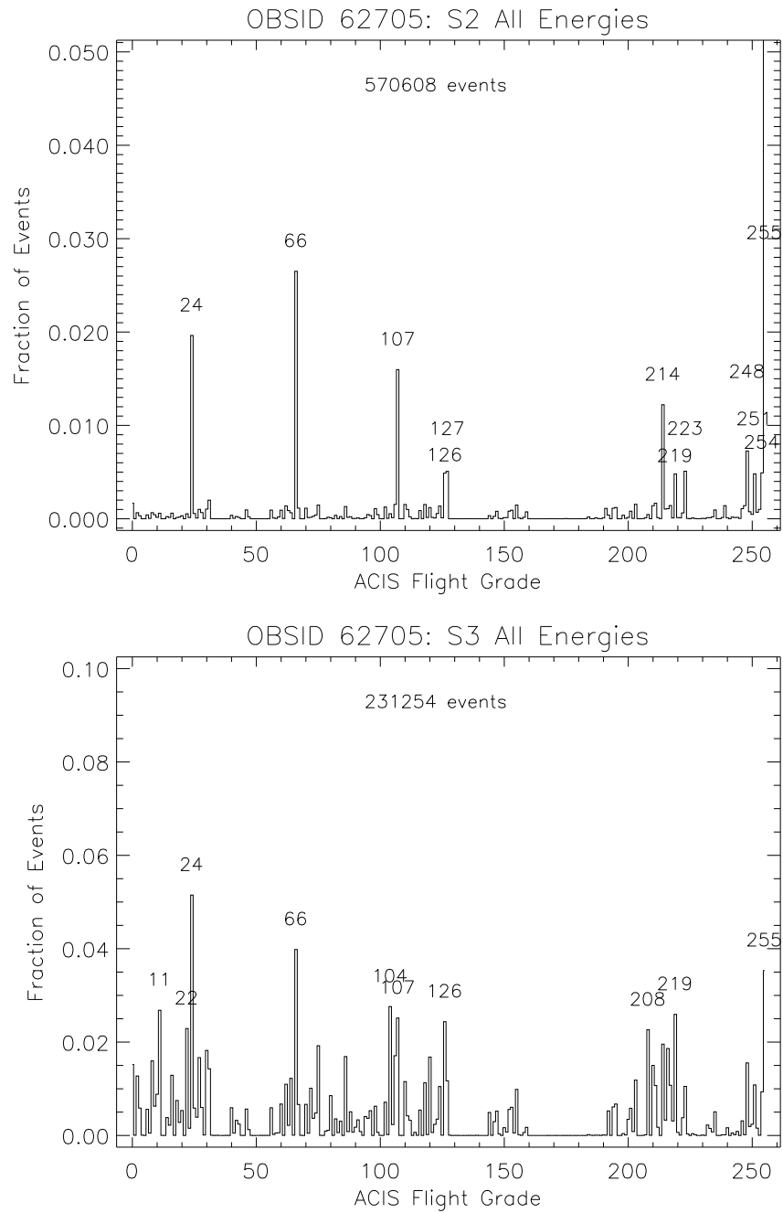
Figure 6.26: Fraction of ACIS background events as a function of grade from early in-flight data for an FI chip (S2) (top) and a BI chip (S3) (bottom).
