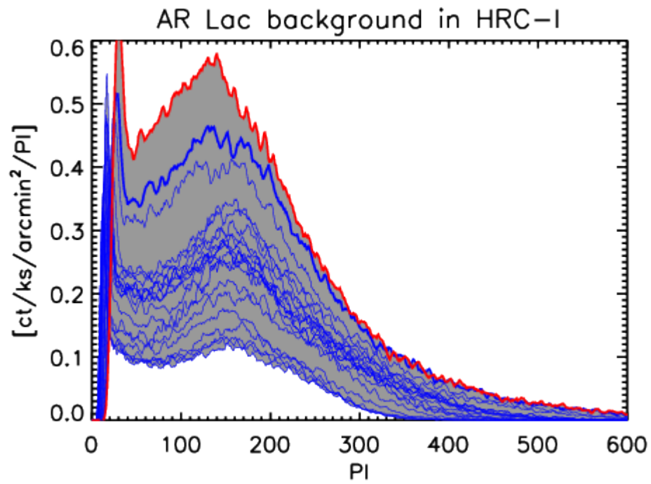
Figure 7.19: Average background PI spectra in the inner 10' region of the detector, obtained from yearly observations towards AR Lac are shown. Times of high background flaring have been excluded. The magnitude and shape of the spectra vary considerably with time, but may be interpolated between epochs to estimate the background for any given observation.
