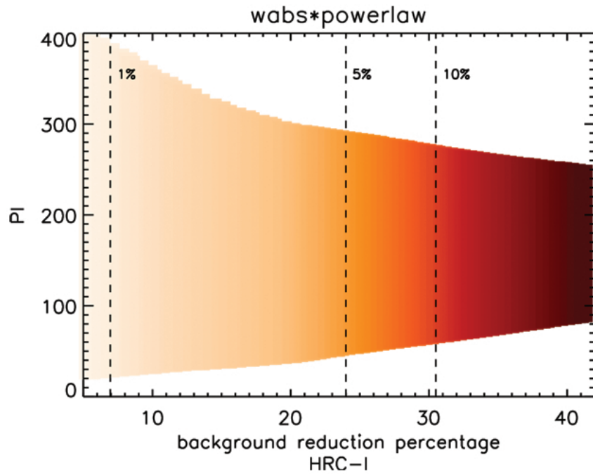
Figure 7.21: The range of PI that should be included to reduce the background by a given percentage is shown in the figure as a shaded band for an assumed absorbed power-law spectrum. All of the parameters included in the grid for Figure 7.9 are considered possible, and these PI ranges can be shrunk if more information is available for a particular source. The depth of the shading indicates how much of the source events are expected to be lost. The vertical dashed lines indicate the background reduction for source event losses of 1%, 5%, and 10%. As shown in Figure 7.19, the background varies with time. Here, for the sake of definiteness, we use the background from the year 2008.
