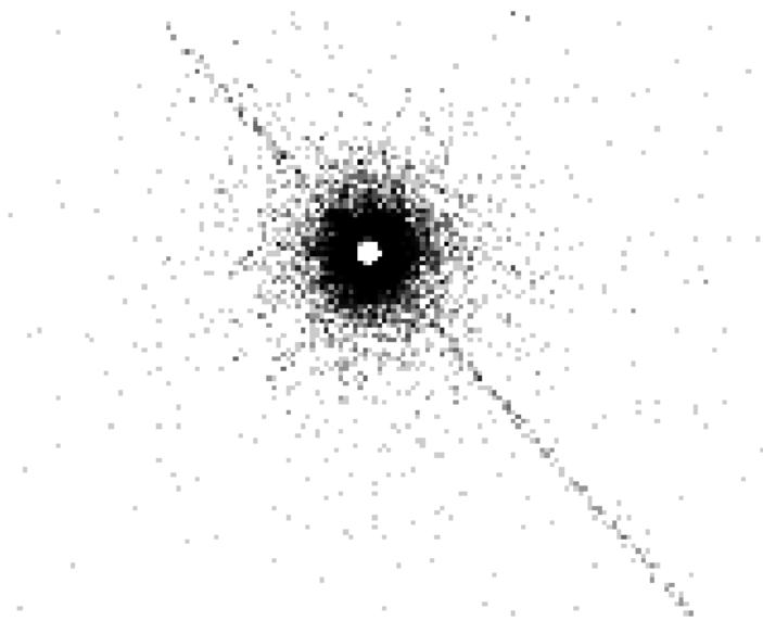
Figure 6.18: Trailed image of a strong X-ray source. The core of the image is faint due to pile-up. Most events here are rejected because of bad grades. The read-out direction is parallel to the trail.
