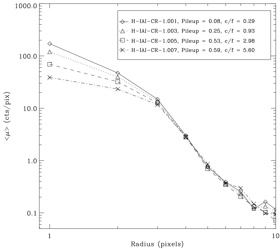
Figure 6.21: The effects of pile-up on the radial distribution of the PSF are illustrated. These data were taken during ground calibration at the XRCF. The specific “OBSIDs”, the counting rate per CCD frame (“c/f”), and the “pile-up fraction” as defined in Section 6.16.2 are given in the inset.
