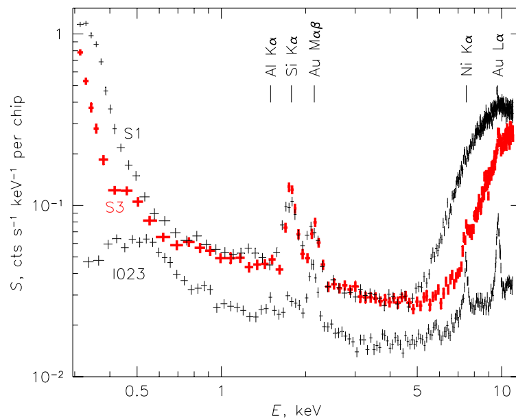
Figure 6.25: Energy spectra of the charged particle ACIS background with ACIS in the stowed position (a 50 ks exposure taken in 2002-Sep; standard grade filtering, no VF filtering). Line features are due to particle-induced fluorescence of material in and surrounding the focal plane.
