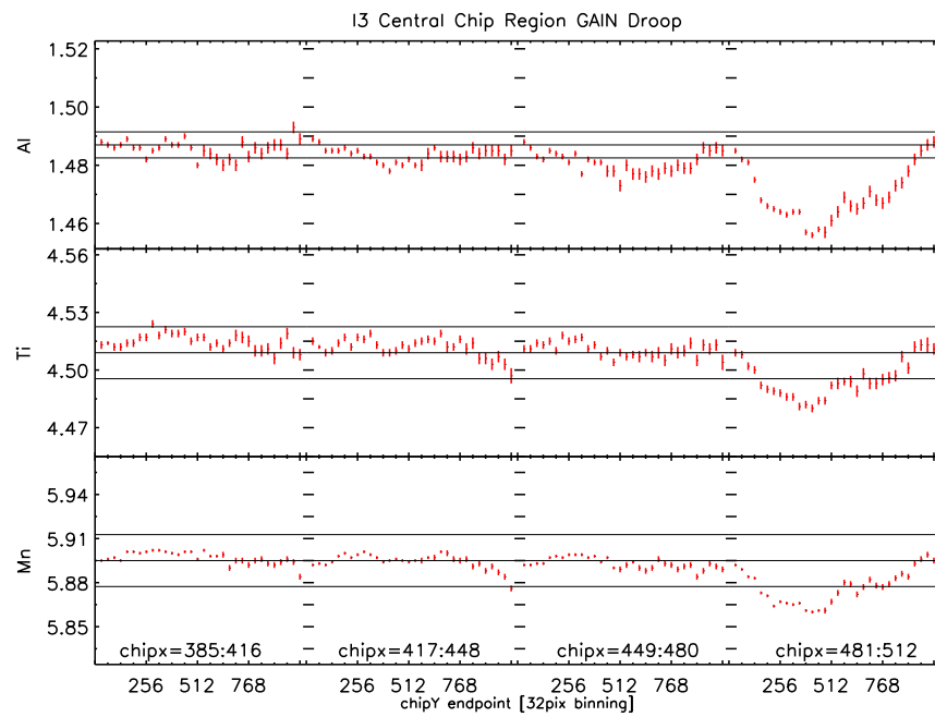
Figure 6.14: Example of the “gain droop” phenomenon seen on FI chips. The energies for three calibration lines are plotted vs CHIPY (32-pixel binning) for four 32-pixel wide (CHIPX) regions adjacent to the node boundary at CHIPX 512, 513.
