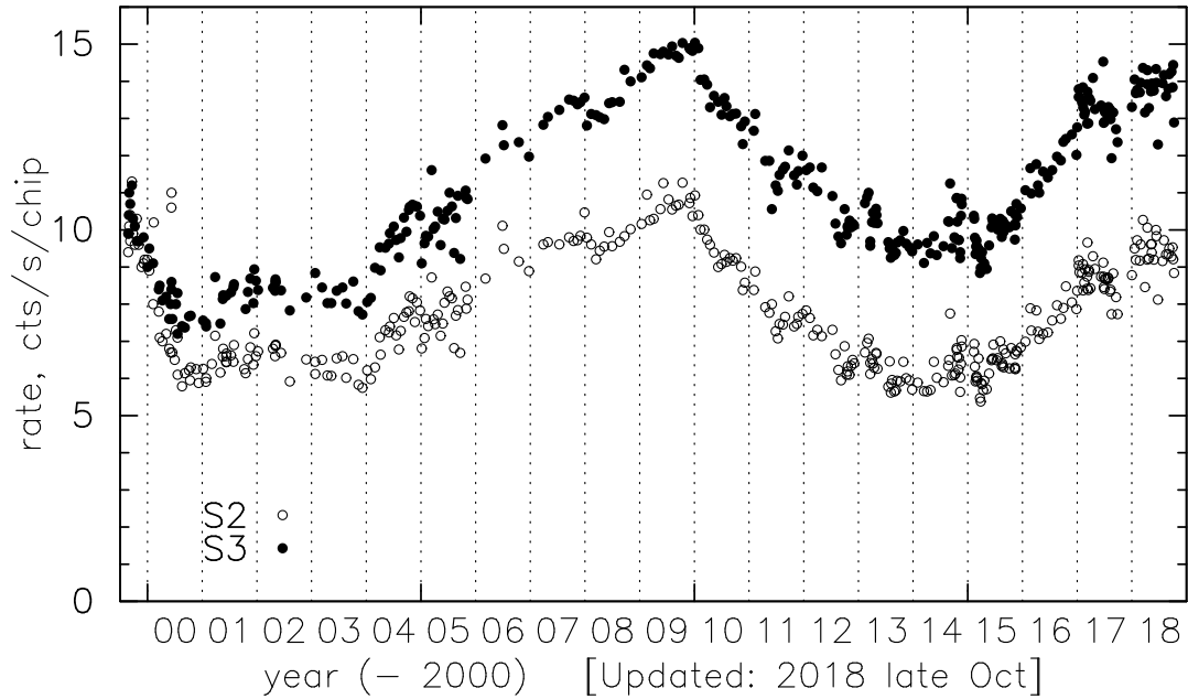
Figure 6.28: Total telemetered background rates (including all grades and the upper event cutoff at 15 keV) for chips S2 (FI) and S3 (BI) as a function of time. Vertical dashed lines are year boundaries. Data are plotted through early October 2018. Beginning in Cycle 11 (late 2009) the default high energy limit was changed from 15 keV to 13 keV. Subsequent 15 keV rate estimates were scaled from 13 keV rates using 13 keV/15 keV conversion factors of 0.82 for S2 and 0.68 for S3. These factors were determined from observations with fairly constant background rates between 2009-Apr and 2009-Jul when the onboard high energy limit was set either to 15 keV or to 13 keV. (See http://cxc.harvard.edu/cal/Acis/detailed_info.html#background for the most recent version of this figure.)
