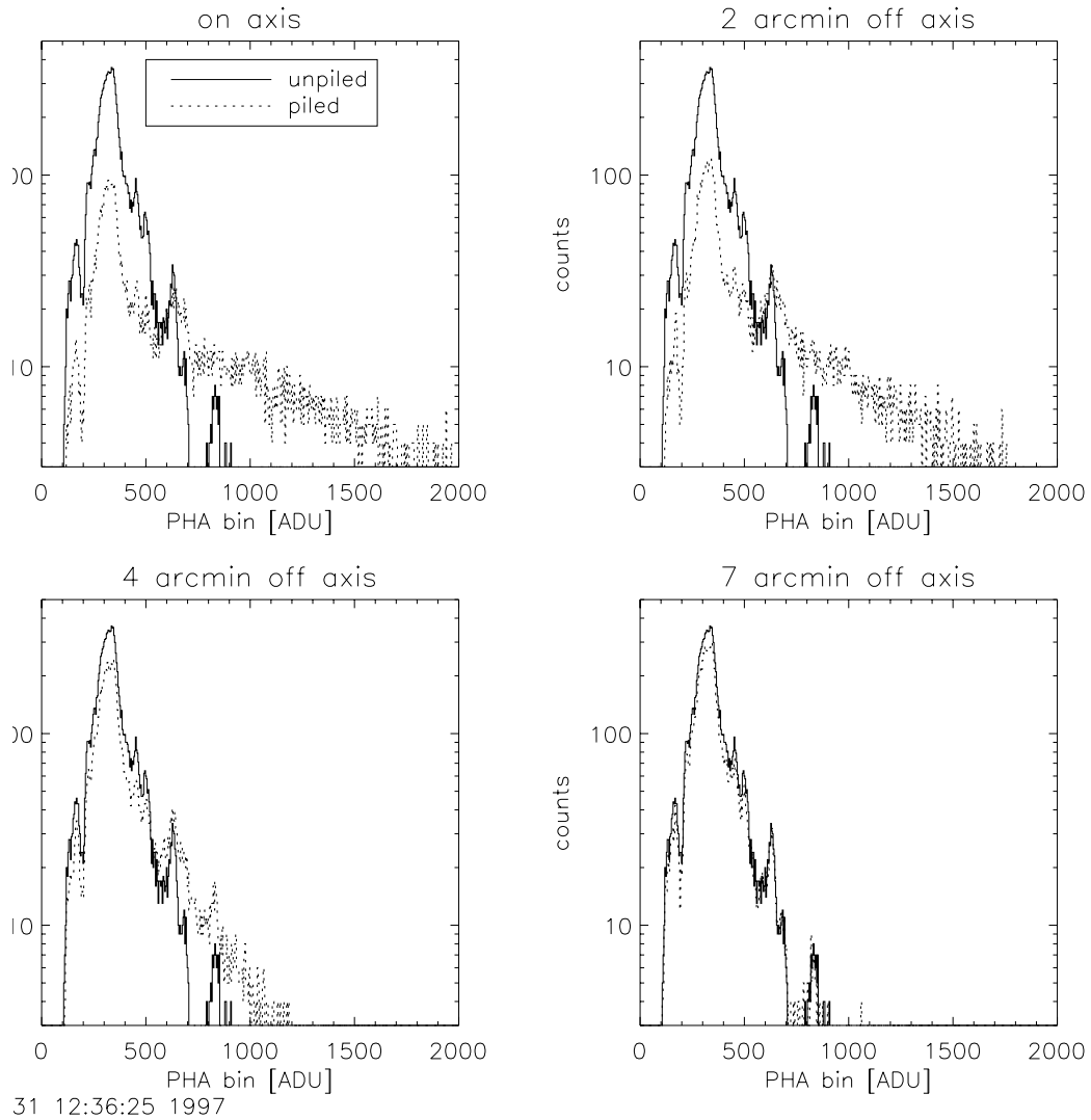
Figure 6.23: MARX simulations of the effect of pile-up on the shape of the spectrum. The true (solid line) and the detected (dotted line) spectra are shown for four different viewing angles. The corresponding “pile-up fractions” – see Section 6.16.2 – are 46%, 40%, 15%, and 2% as the image is moved progressively further off-axis.
