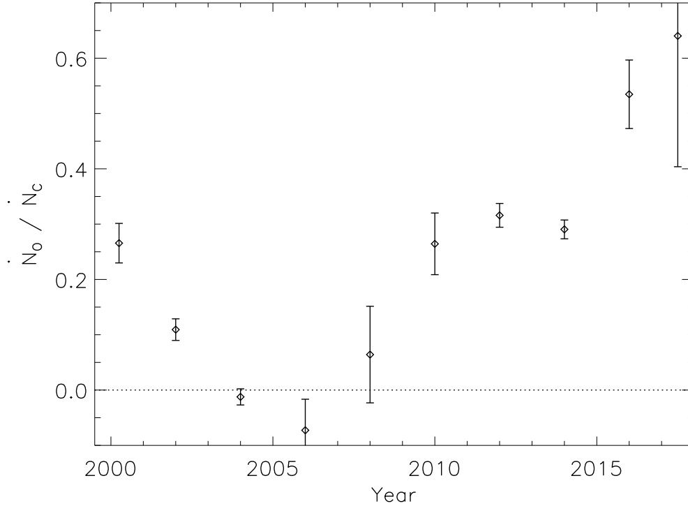
Figure 6.9: The ratio of the deposition rate in oxygen atoms per year to that for carbon over the Chandra mission as measured by LETG/ACIS-S observations of blazars.
