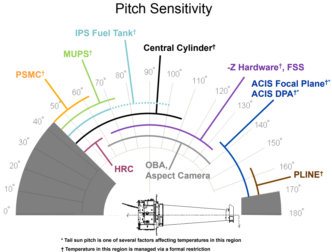
Figure 6.32: Pitch sensitivity of spacecraft components
