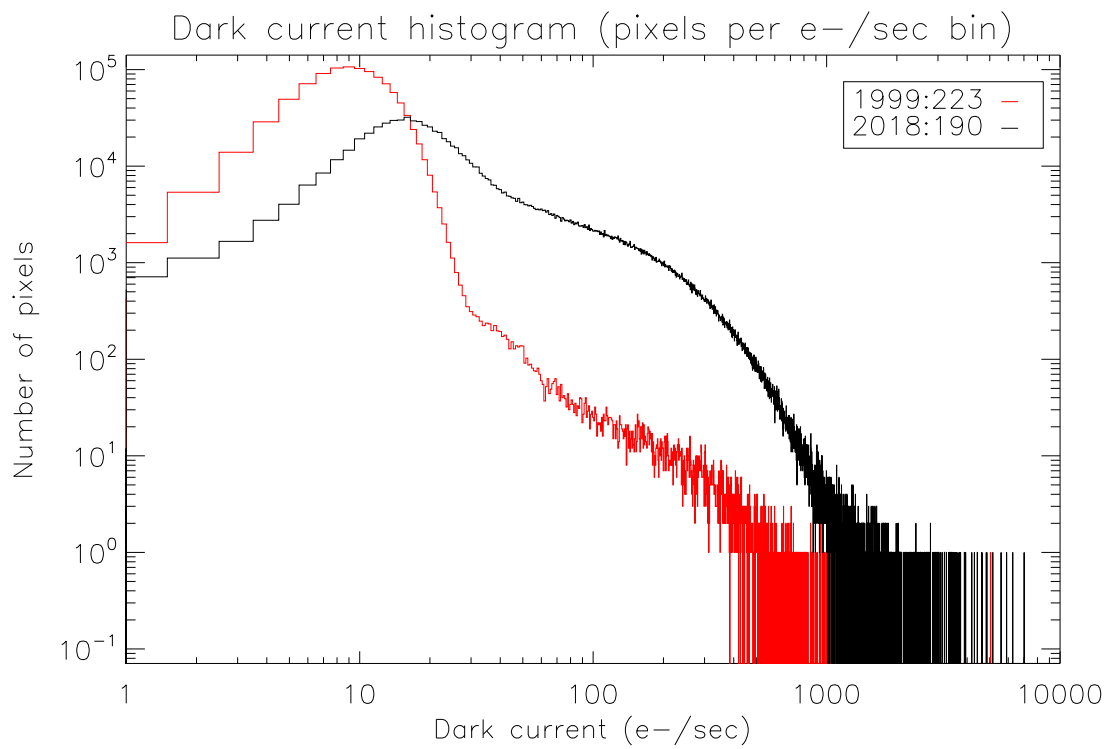
Figure 5.8: Differential histogram of dark current distribution for the ACA CCD in 1999-Aug and 2018-July
