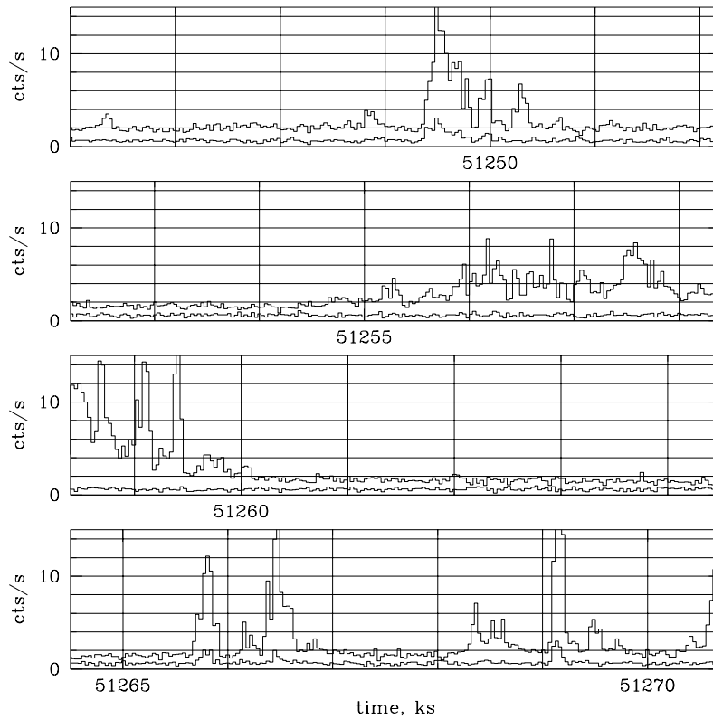
Figure 6.29: An example of the ACIS background counting rate versus time – BI chip (S3; top curve) and an FI chip (I2; bottom curve). These are for the standard grades and the band from 0.3 - 10 keV.
