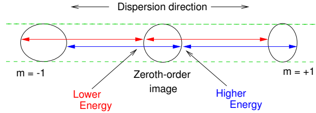
Figure 8.28: HETGS spatial-spectral effect example. In this schematic, a zeroth-order ring image emits at an energy which varies across the ring’s diameter in the dispersion direction emitting lower-energy photons on the left and higher-energy photons on the right. The resulting diffracted images in \pm 1 st orders have different appearances due to the spatial-spectral interaction. In the cross-dispersion direction, however, the images have the same extent.
